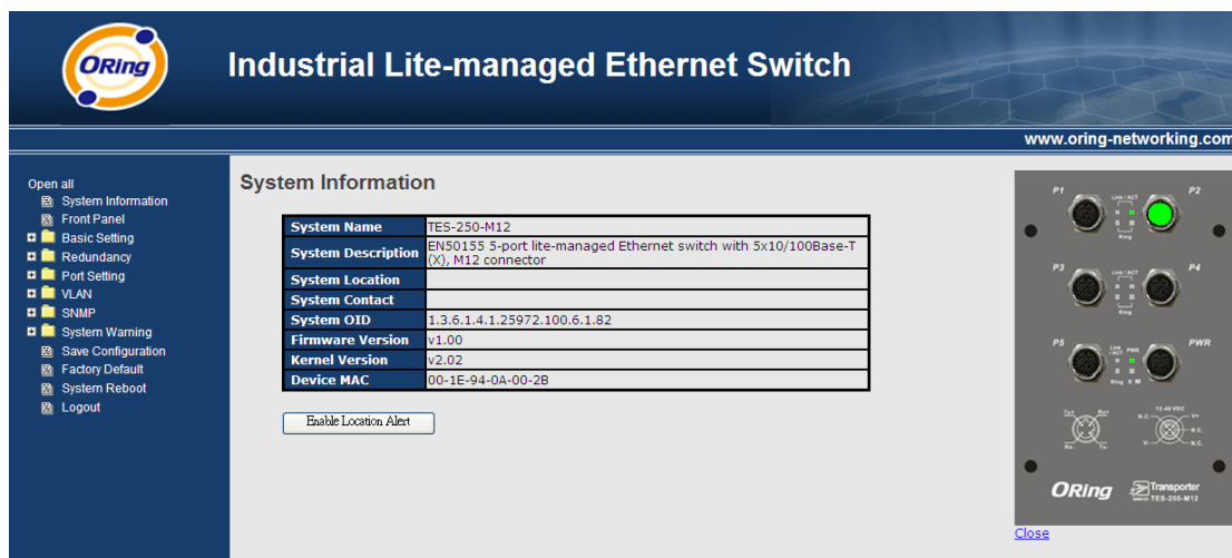
Main interface
