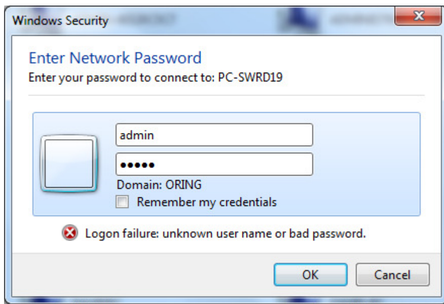
Login screen
