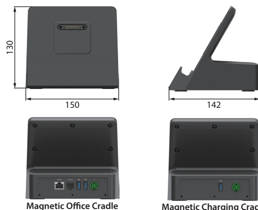
Magnetic Office Cradle
