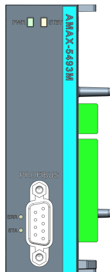
Figure 5.11 AMAX-5493M Module LED Indicator
