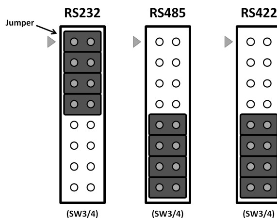
Figure 5.7 AMAX-5490 SW3/SW4
