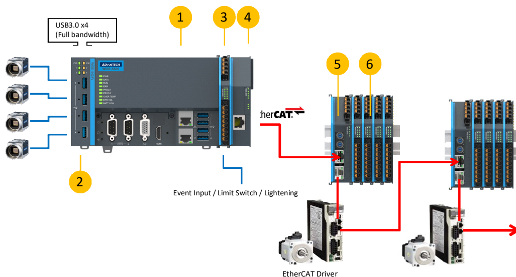
Figure 2.5 AMAX-5000 System Configuration for Motion + Vision Application
