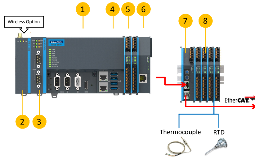
Figure 2.6 AMAX-5000 System Configuration for Big Data Edge Concentrator
