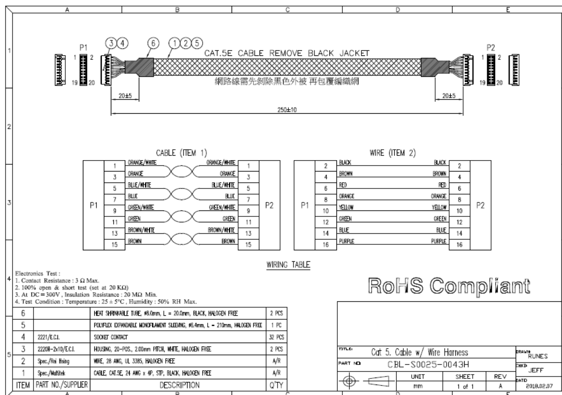
Figure 16: Board to Board LAN Cable Drawing
