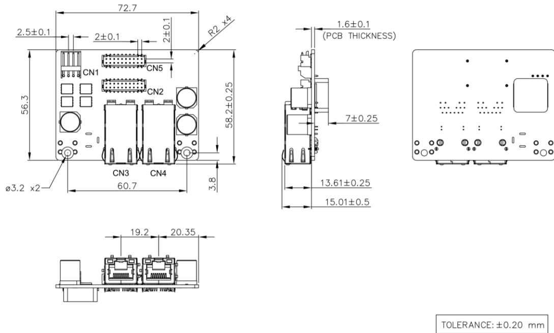
Figure 11: Bracket Daughter Board Drawing - 4Pin Header (EMPL-G2P1-C6/W6)
