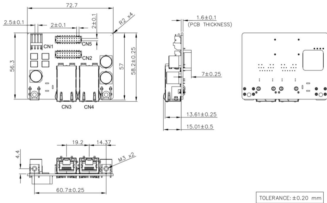
Figure 10: Mounting Hole Daughter Board Drawing - 4Pin Header (EMPL-G2P1-C5/W5)
