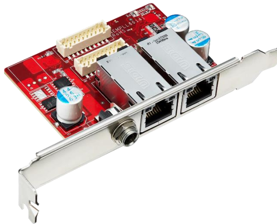
Figure 6: Bracket, DC Jack, Daughter Board Picture (EMPL-G2P1-C8/W8)
