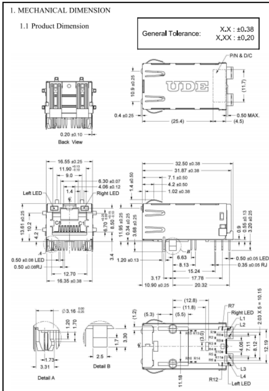
Figure 8: RJ45 Connector Drawing
