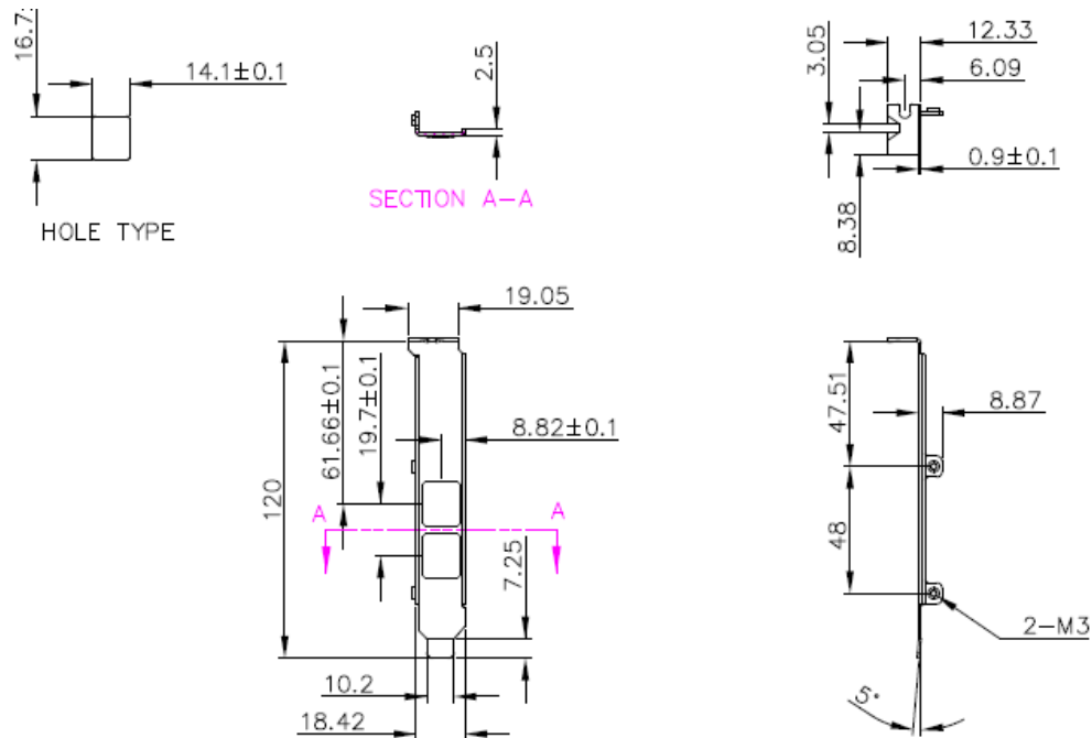
Figure 14: Bracket Drawing
