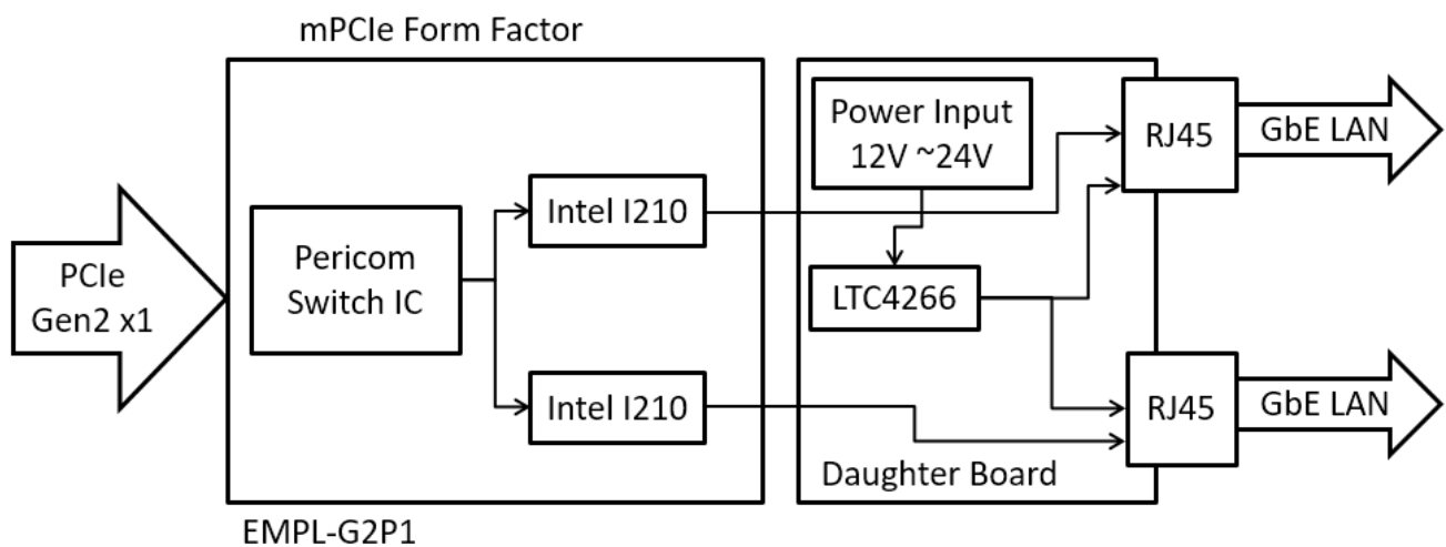
Figure 1: Block Diagram
