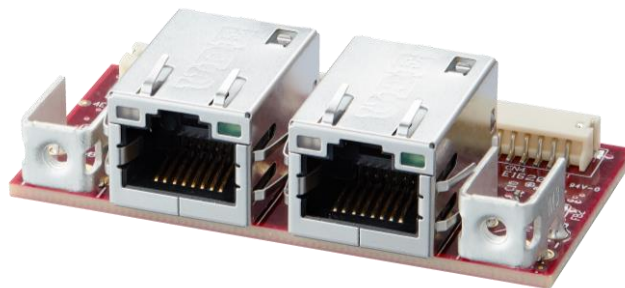
Figure 3: Mounting Hole Daughter Board Picture (EMPL-G202-C3/W3)
