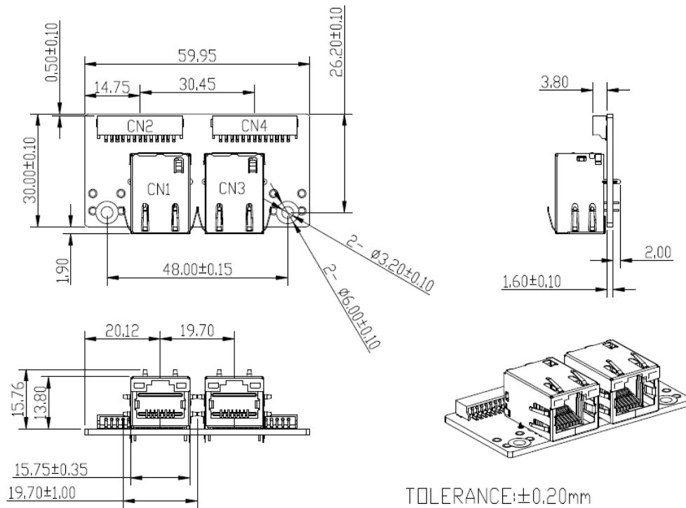
Figure 9: Bracket Daughter Board Drawing (EMPL-G202-C4/W4)
