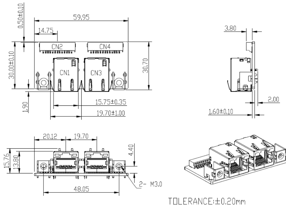
Figure 8: Mounting Hole Daughter Board Drawing (EMPL-G202-C3/W3)
