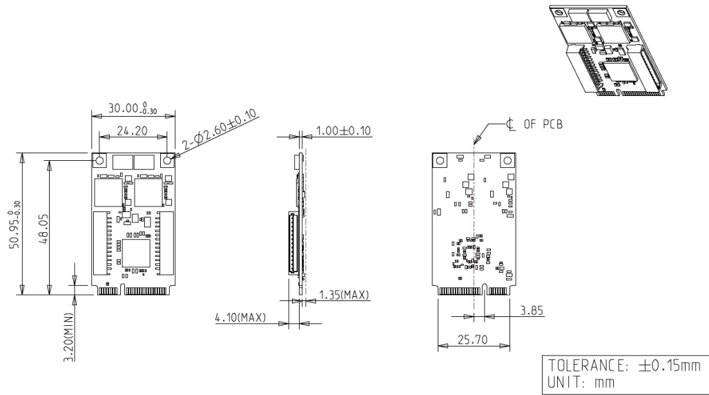
Figure 7: EMPL-G202 mPCIe Board Drawing
