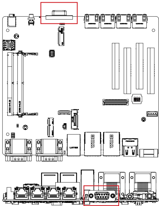
GPIO Connector
