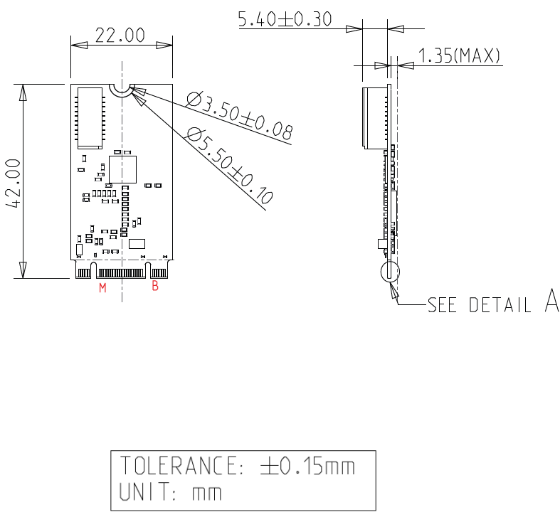
EGP2-X203-W2 (Horizontal Connector)
