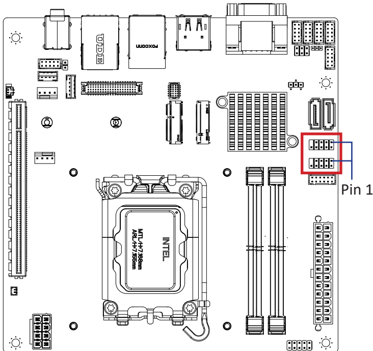
USB 2.0 Header
