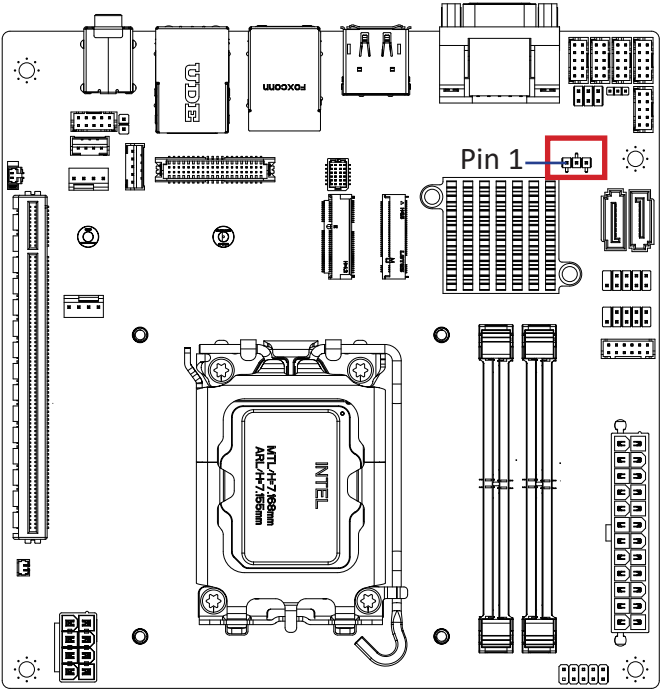
Clear CMOS Jumper
