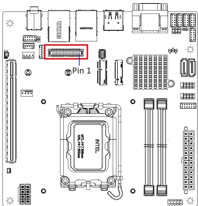
LVDS Connector
