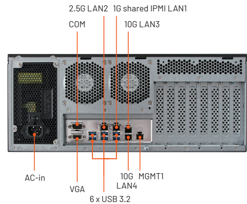
(System Rear I/O)
