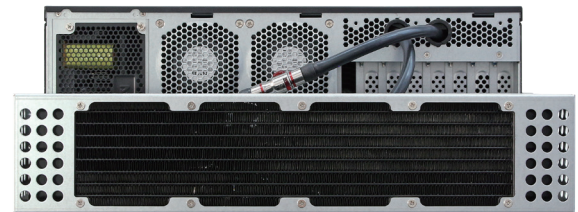
(Rear View of the Installed 1-1 Liquid Cooling Module)
