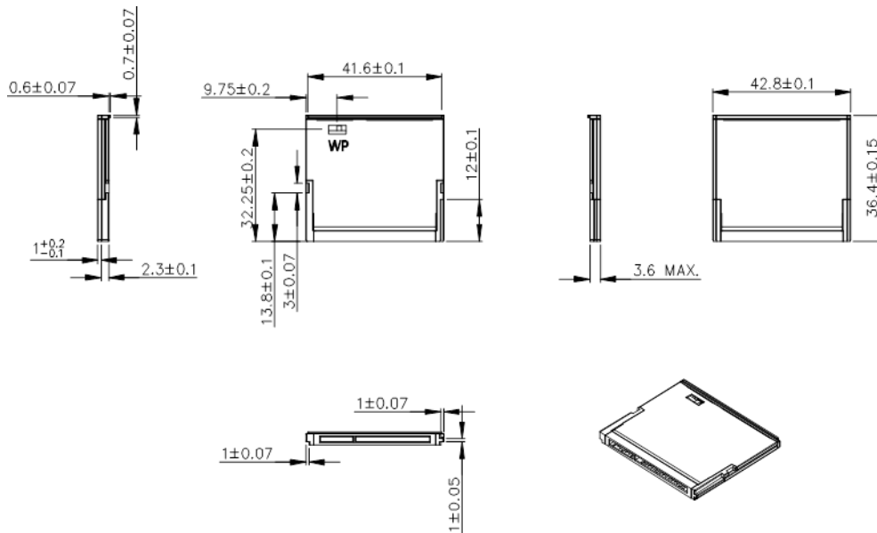
Figure 2: Innodisk CFast 3TE7 diagram
