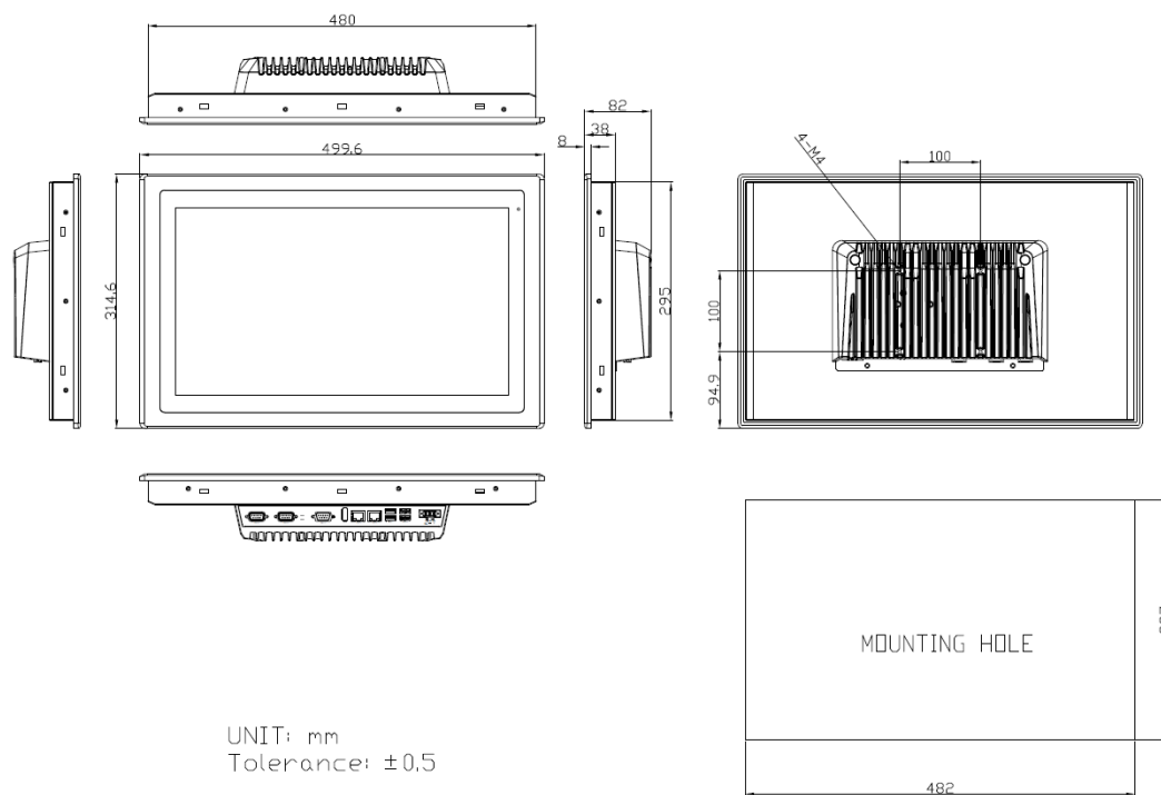
Figure 7 Dimensions of ARCHMI-S-918D P/R(H)
