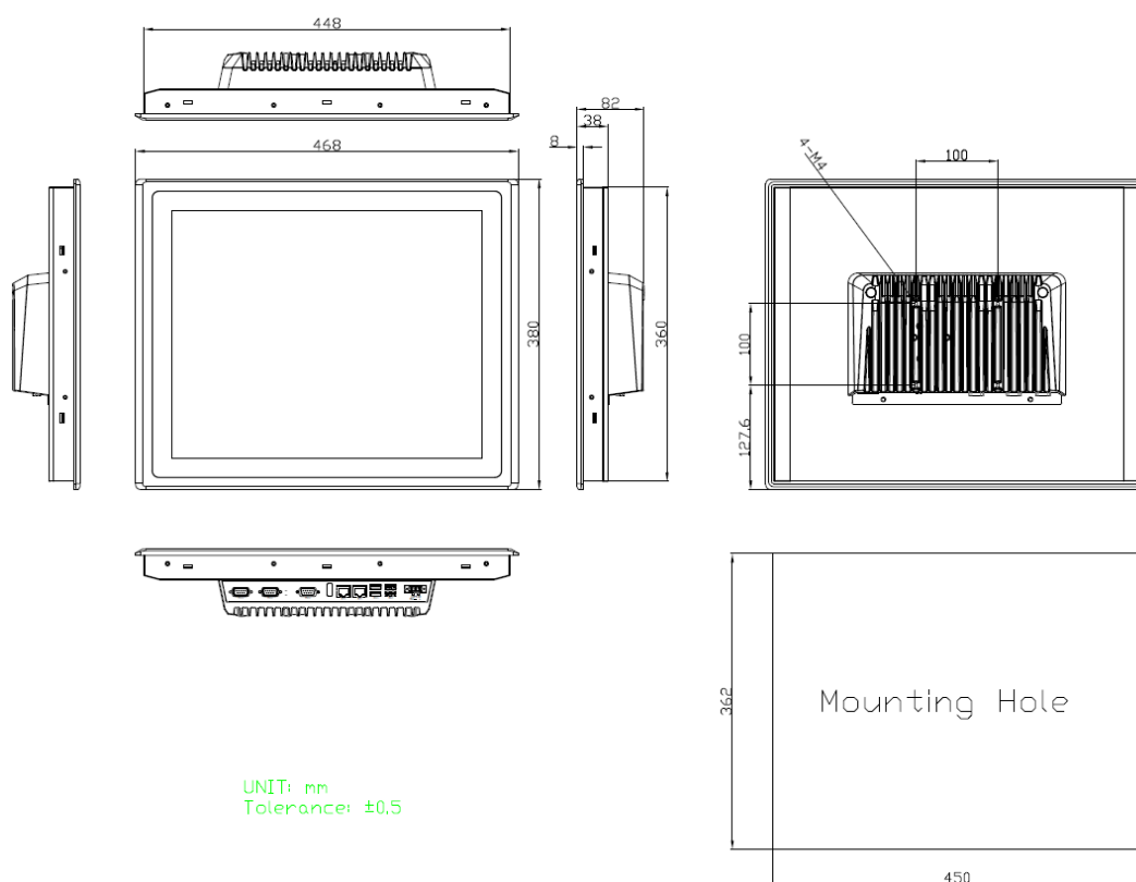
Figure 8 Dimensions of ARCHMI-S-919D P/R(H)
