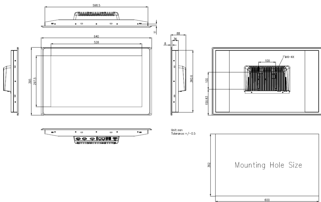
Figure 10 Dimensions of ARCHMI-S-924DP(H)
