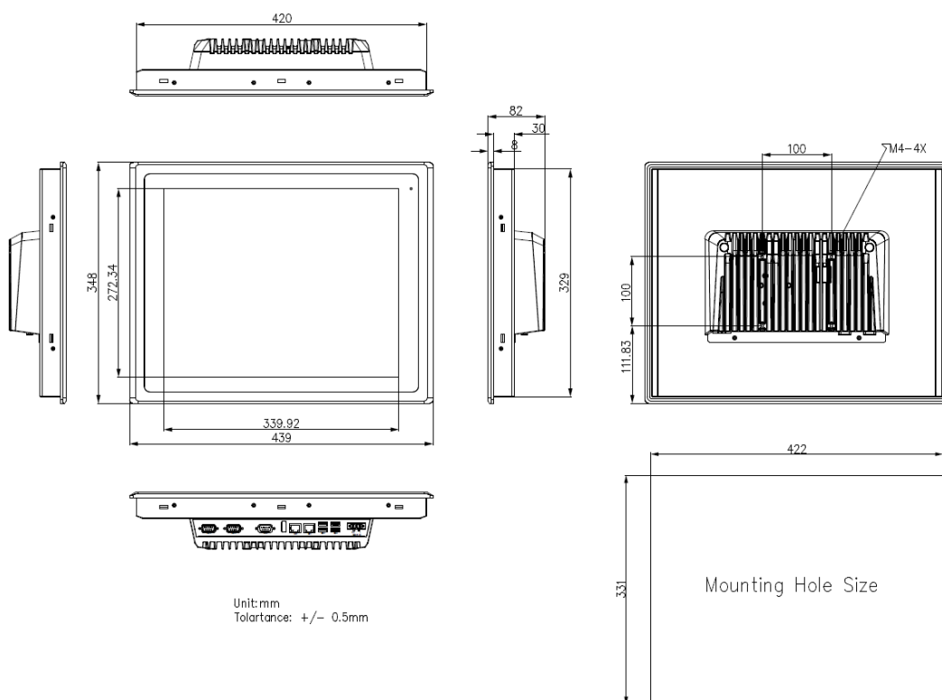
Figure 6 Dimensions of ARCHMI-S-917DP/R(H)
