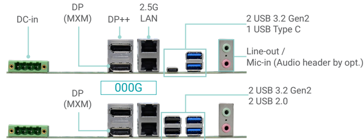
200G Rear View (RPS183-H610E)
