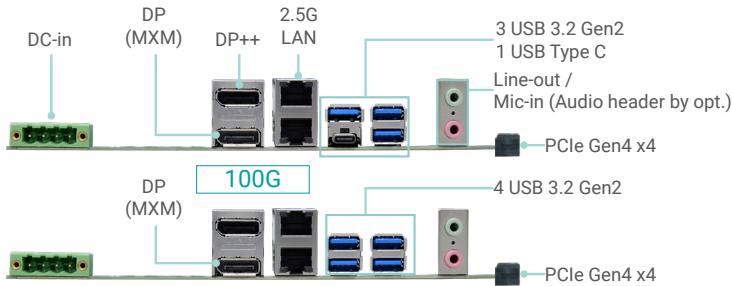
300G Rear View (RPS183-Q670E)
