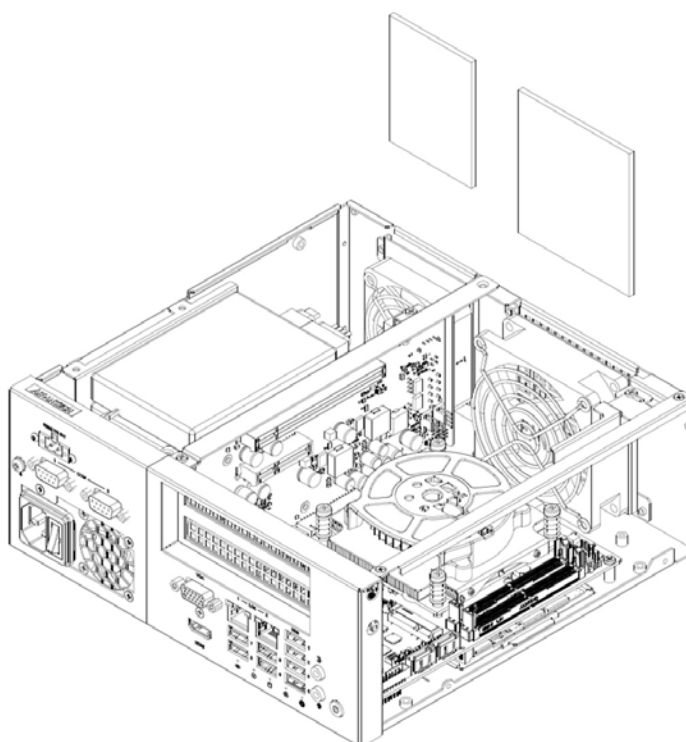
Figure 3.3 Removing the Filters /取出过滤器/取出濾網
