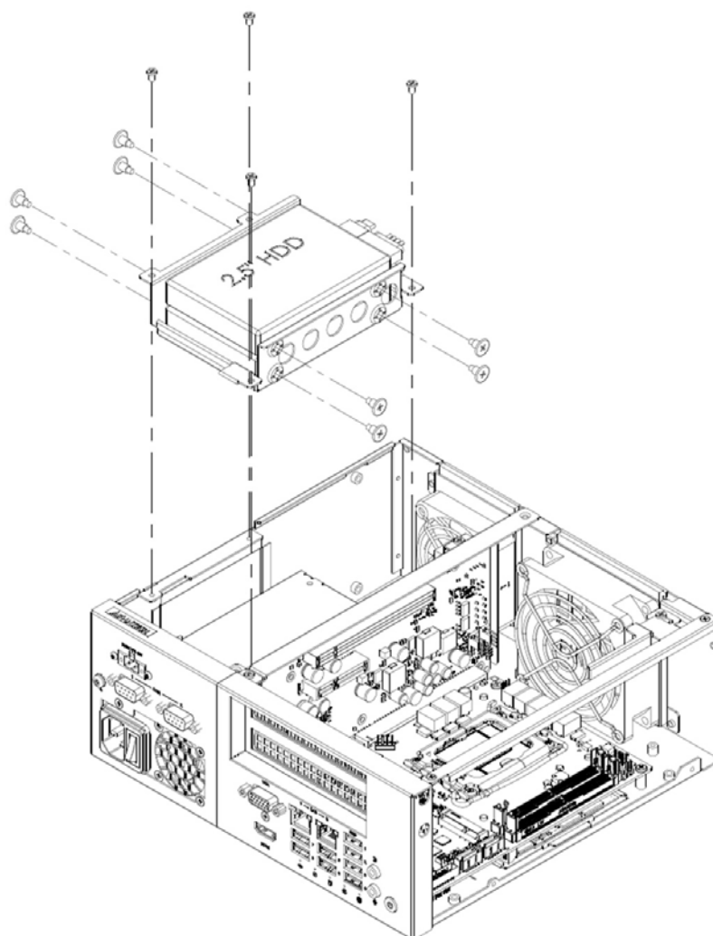
Figure 2.2 Installing internal 2.5" SSD/HDD / 安装2.5" 硬盘/固态硬盘/安装2.5" 硬碟 / 固態硬碟
