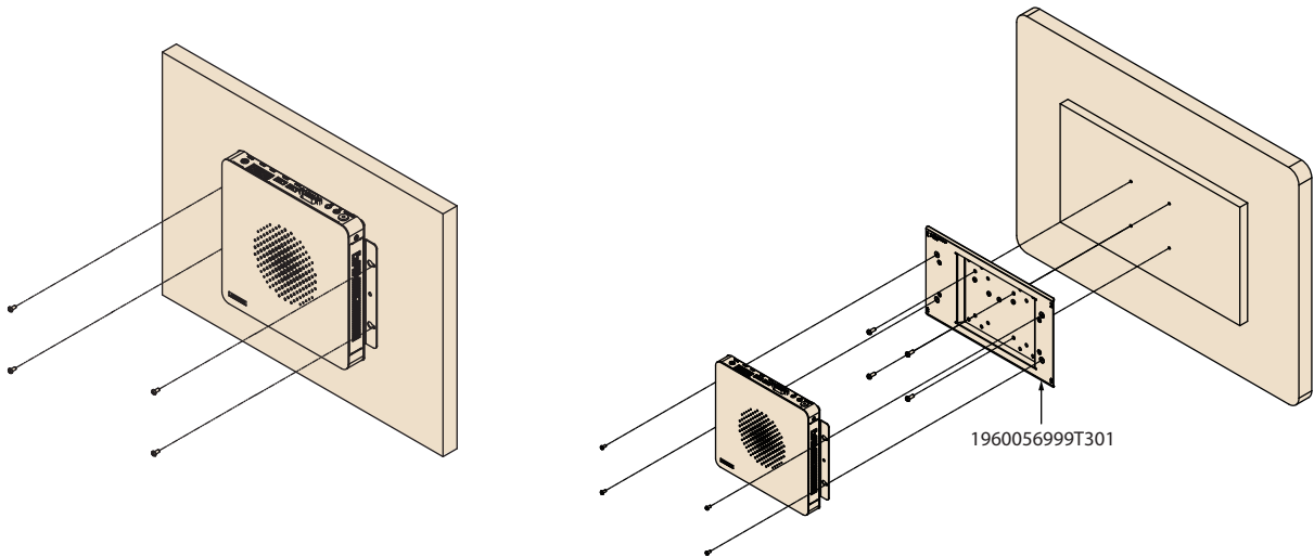
Wall Mount
