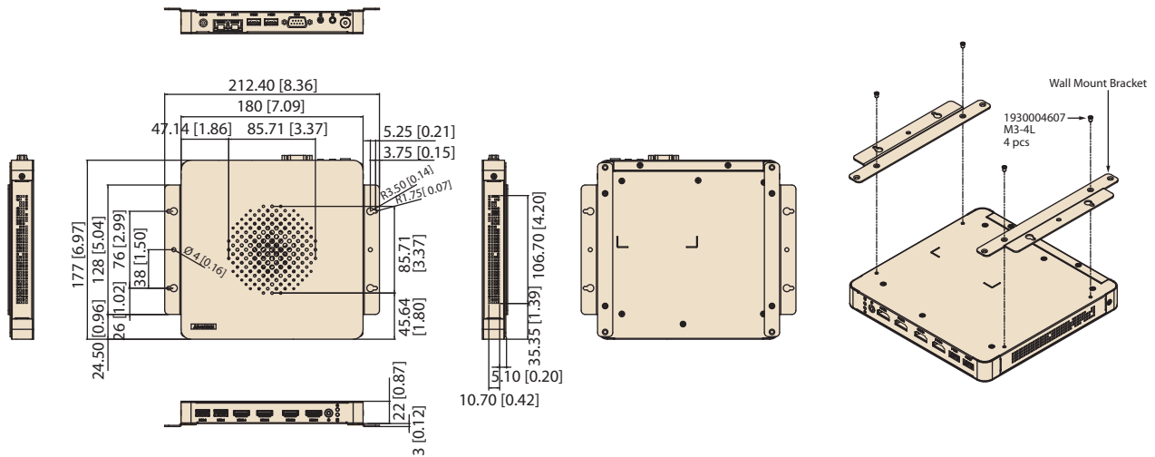
Wall Mount
