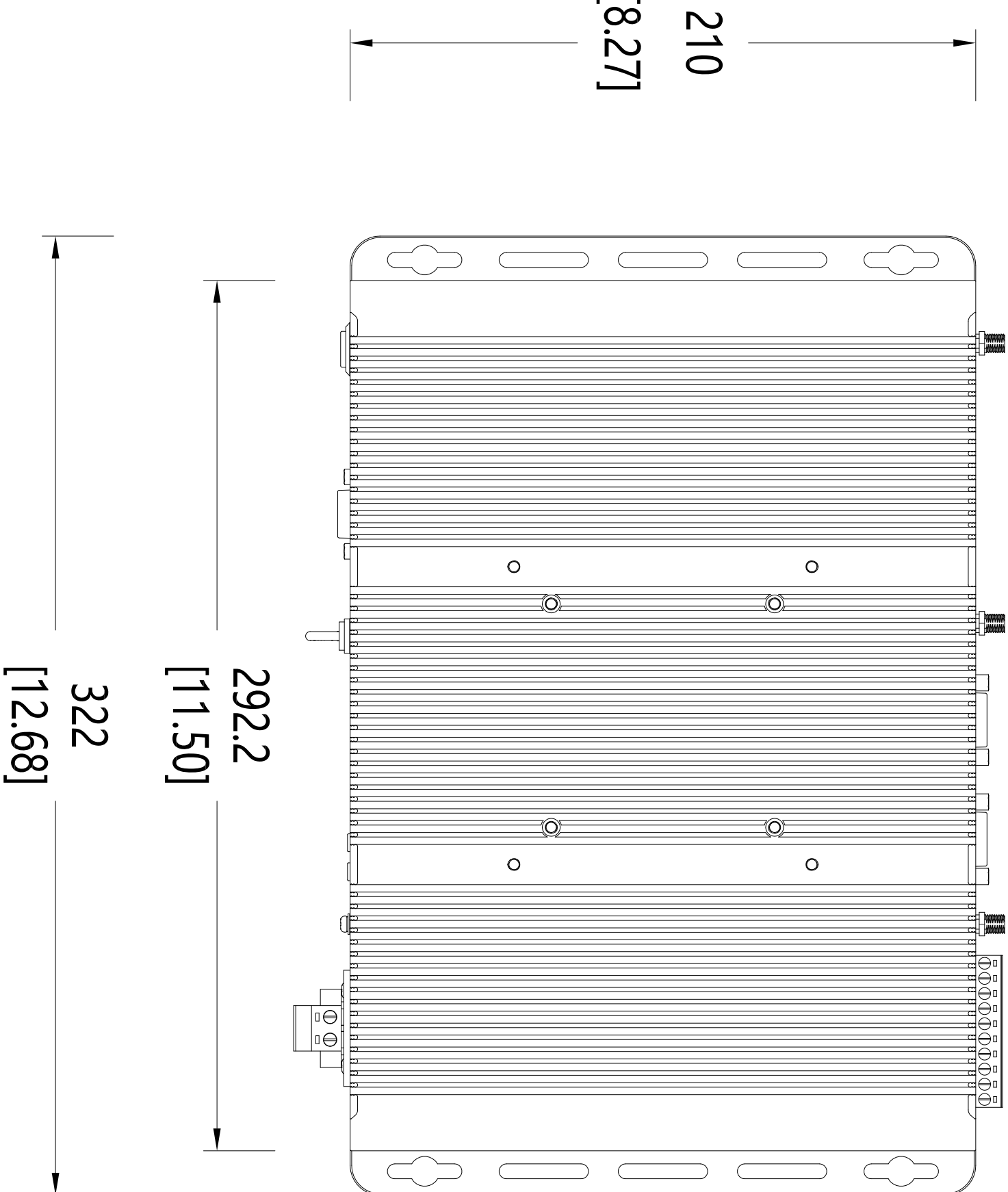
Front View
