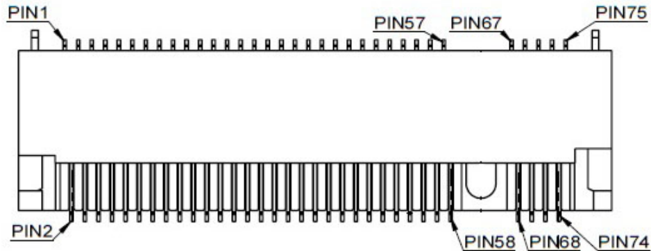
Figure 30: M.2 Key M 2280 Slot M2M1
