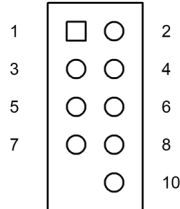
Figure 15: USB 2.0 Port 5, 6 Header CN18, Port 7, 8 Header CN19
