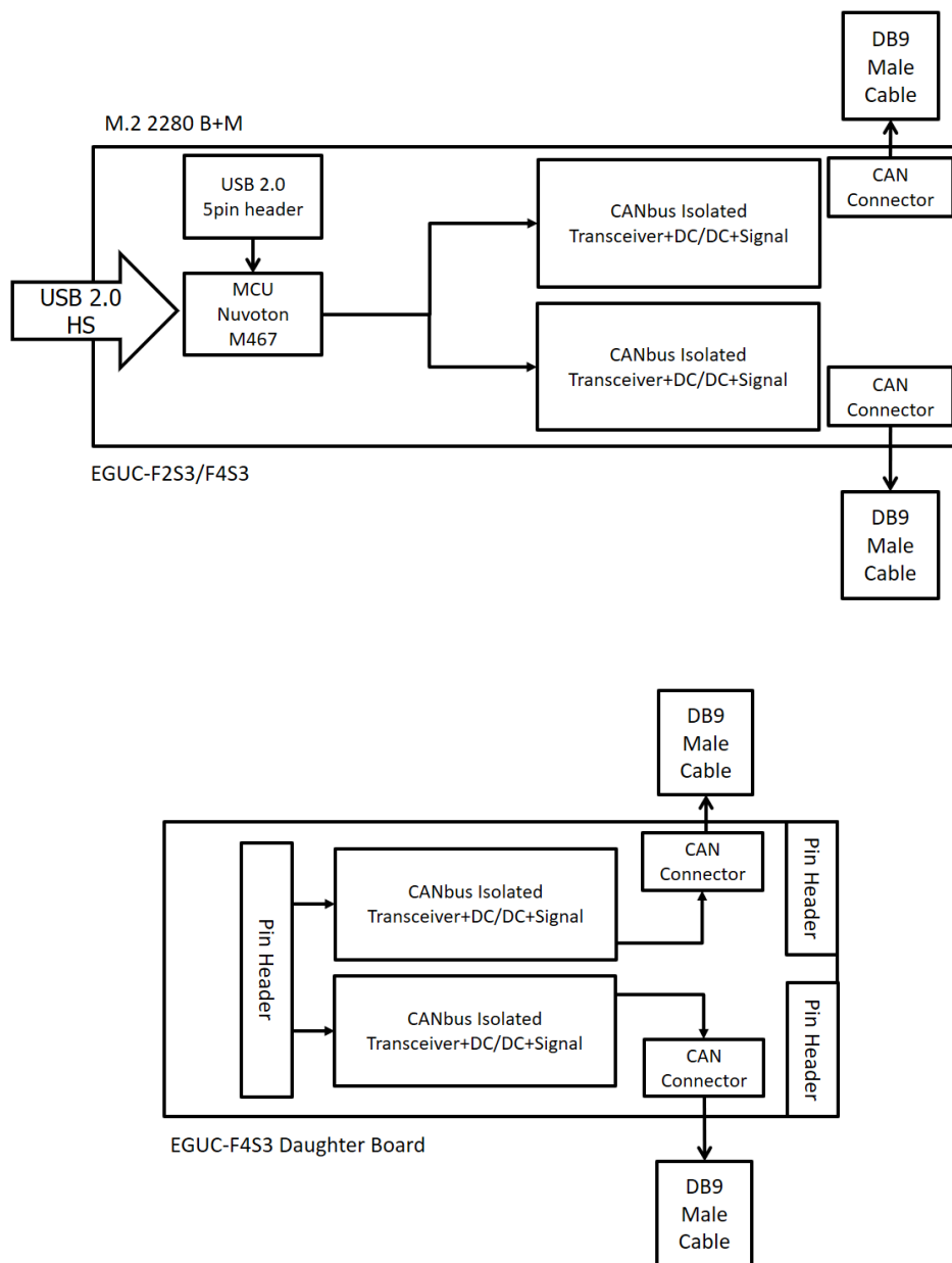
Figure 1: Block Diagram
