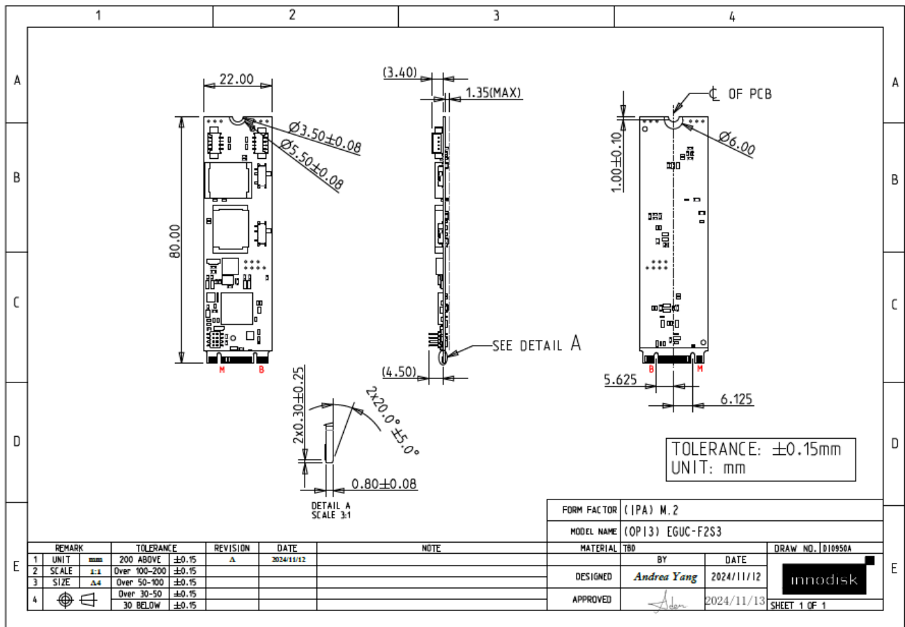
Figure 6: EGUC-F4S3 Drawing
