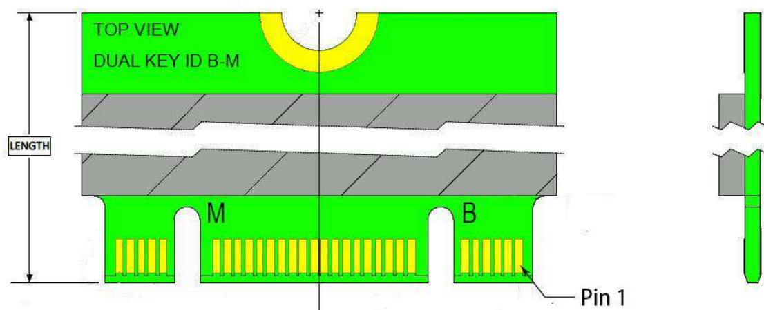
Figure 3-1 SATA Connectors
