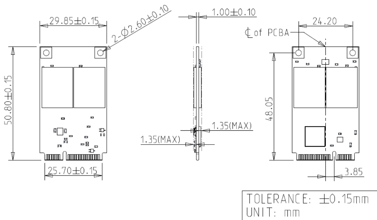
Figure 2: Innodisk mSATA 3TE7 diagram
