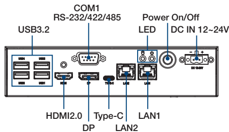
Front Panel External I/O Mechanical Layout/Drawing
