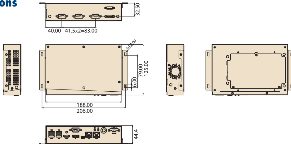
Front Panel External I/O Mechanical Layout/Drawing
