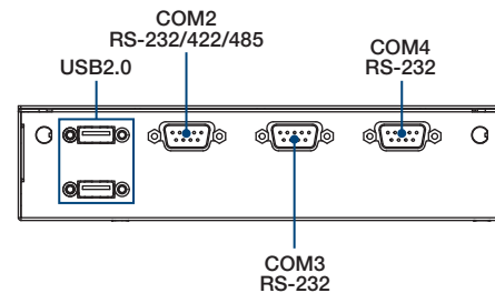
Rear Panel External I/O Mechanical Layout/Drawing
