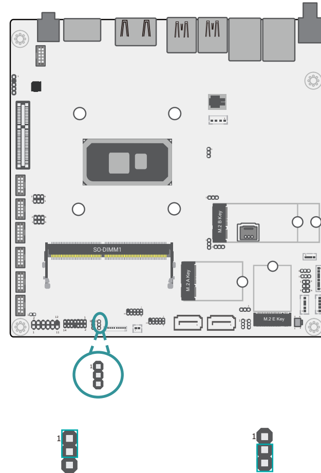
DIO_4~7 Power Select (JP5)
