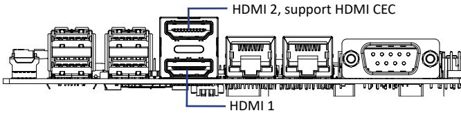
HDMI Connector
