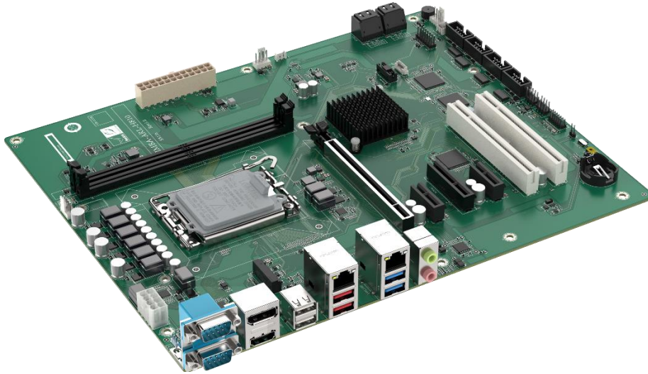
Figure 1-1: IMBA-ARL-H810
