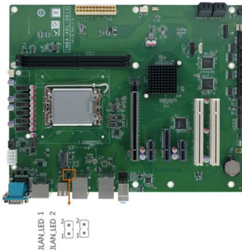
Figure 3-16: LAN LED Connector Locations
