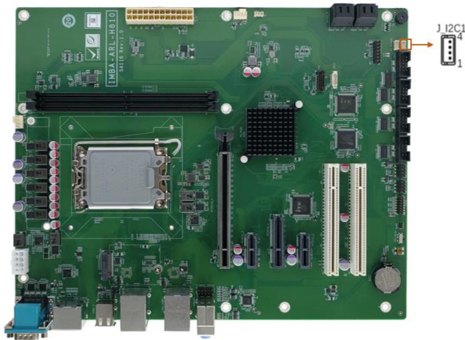
Figure 3-15: I 2 C Connector Location
