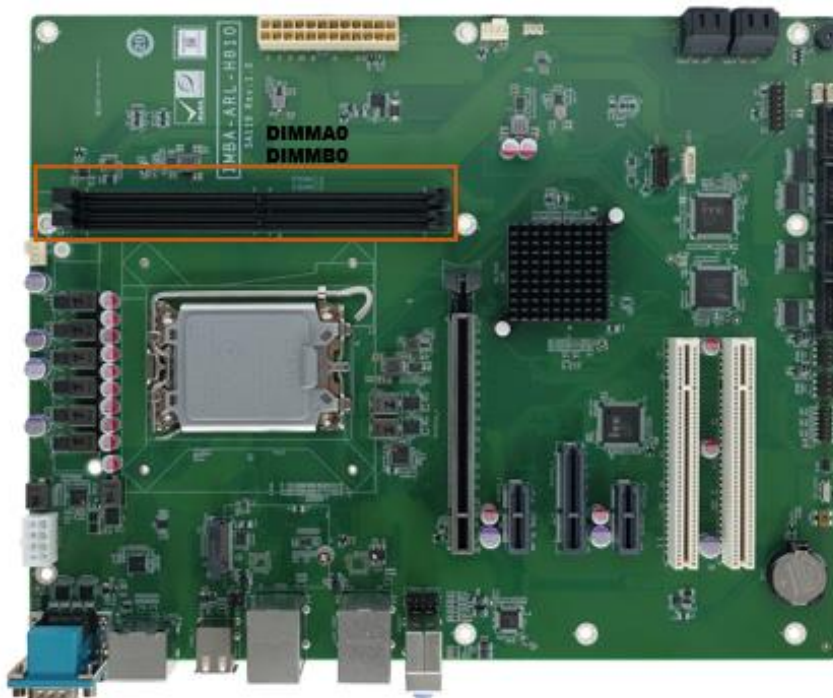
Figure 3-10: DDR5 UDIMM Sockets Location
