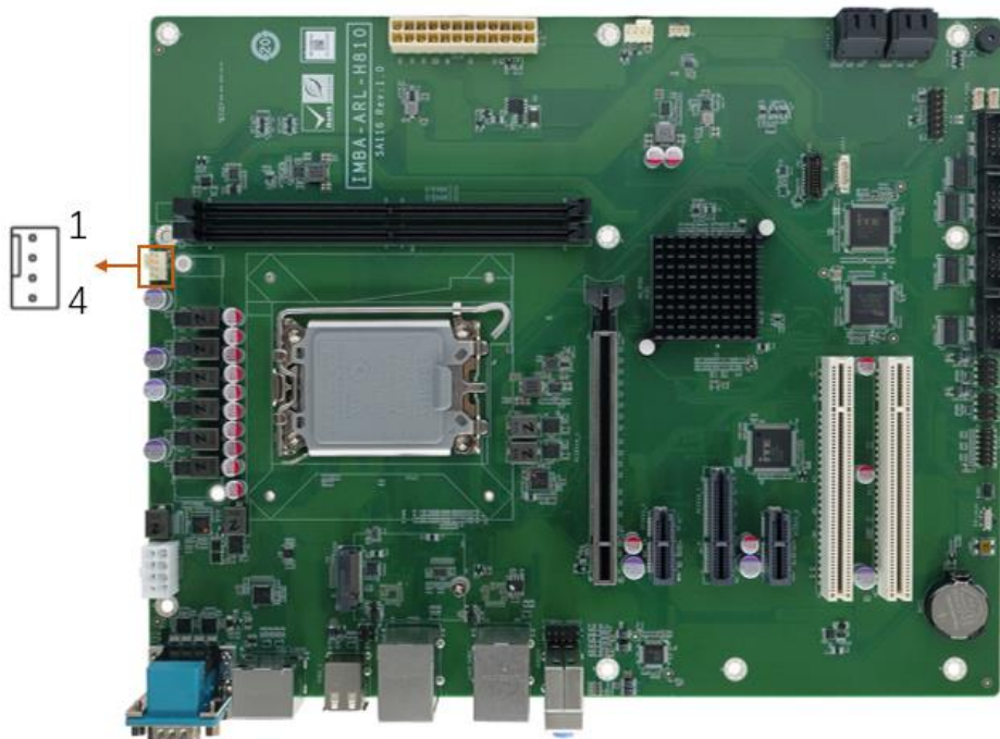
Figure 3-12: CPU Fan Connector Location
