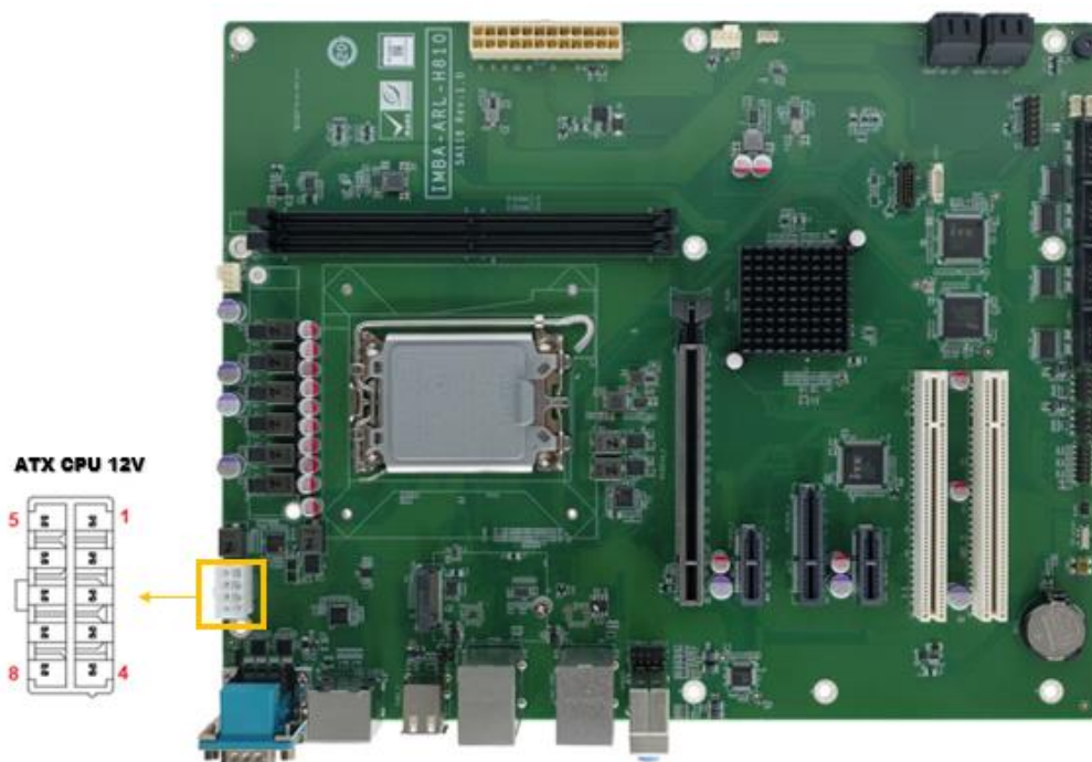
Figure 3-2: ATX CPU 12V power connector location
