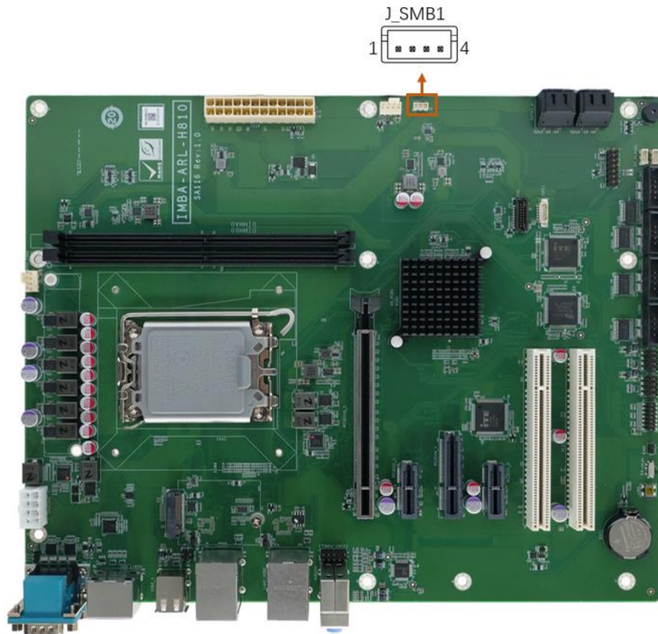
Figure 3-19: SMBus Connector Location
