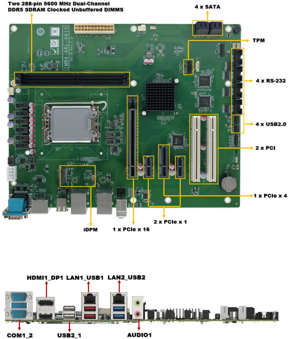
Figure 1-2: Connectors
