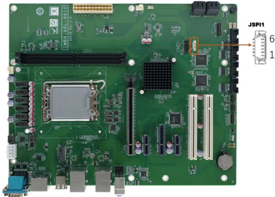
Figure 3-20: Flash SPI ROM Connector Location
