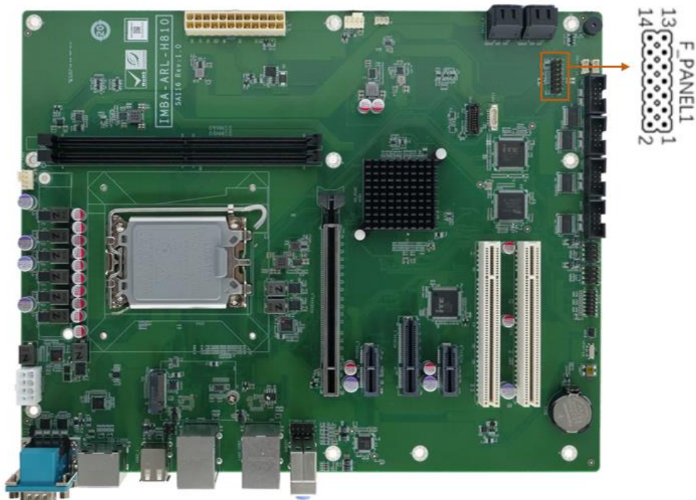
Figure 3-14: Front Panel Connector Location
