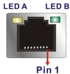
Figure 3-30: LAN LED Location
