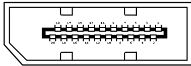
Figure 3-29: DP++ Connector
