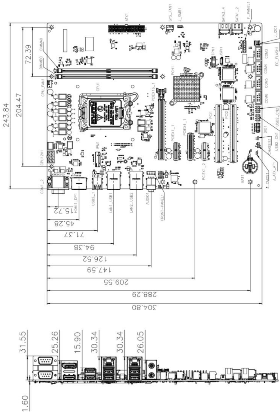
Figure 1-3: IMBA-ARL-H810 Dimensions (mm)
