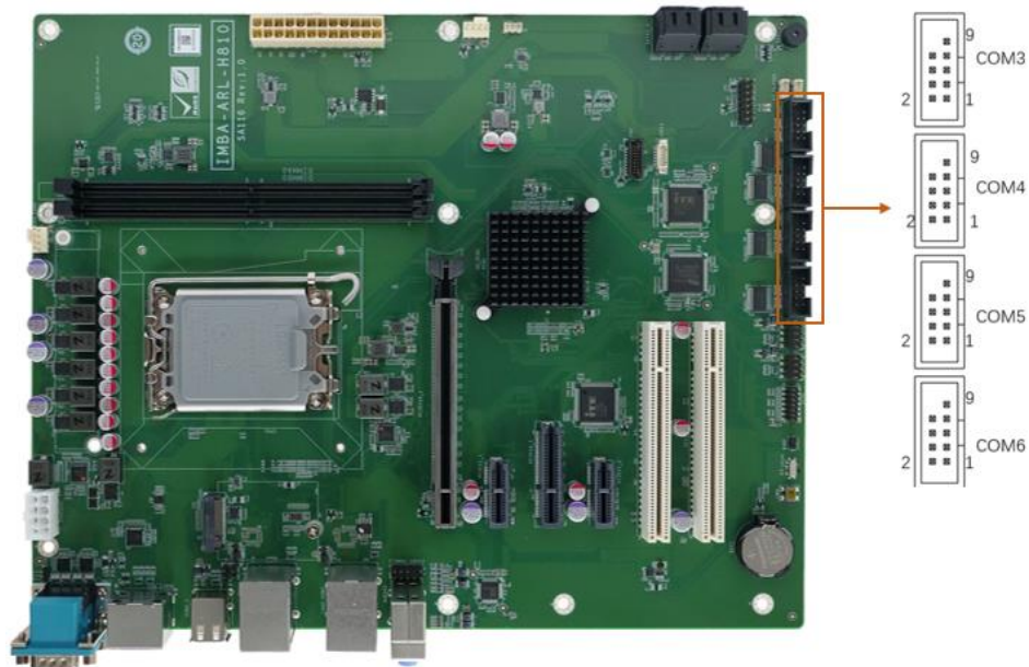
Figure 3-17: RS-232 Serial Port Connector Location
