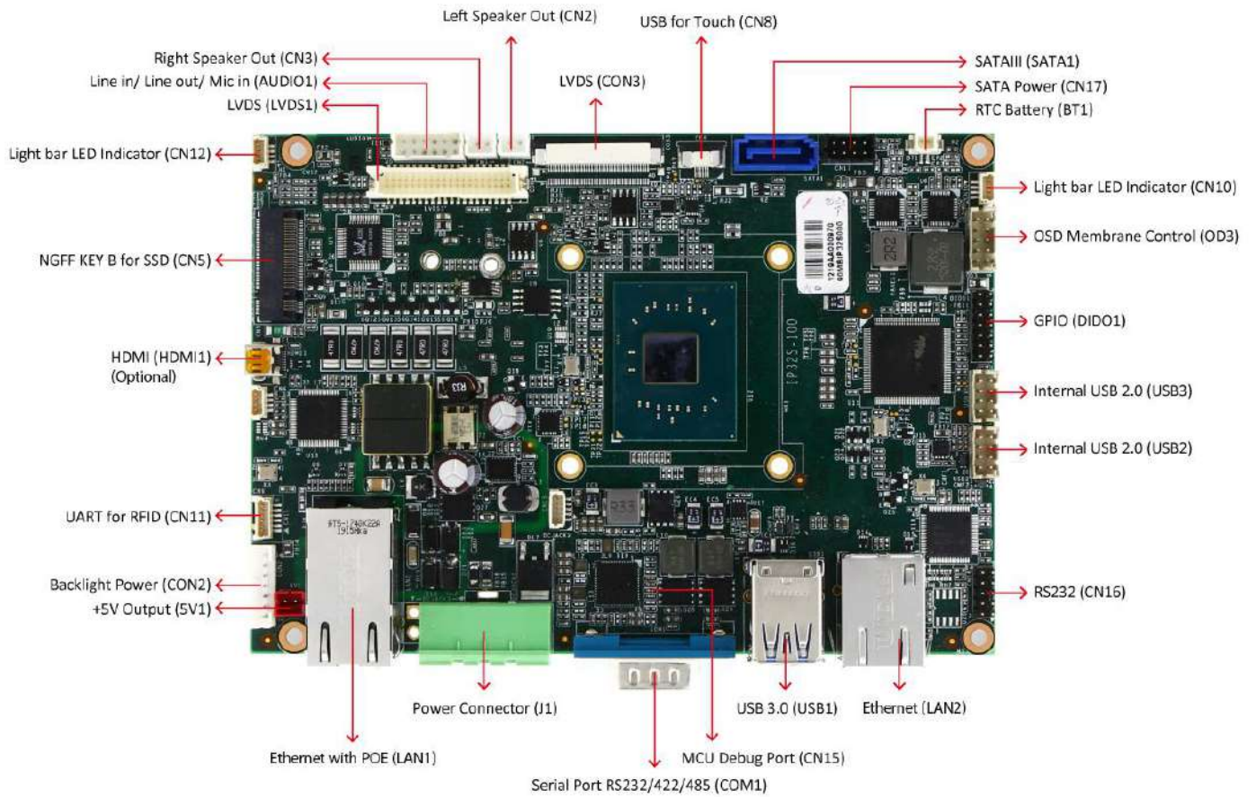
PCB Top Layer (Top View)
