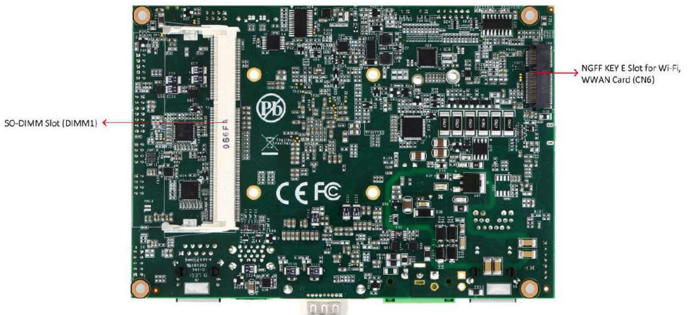
PCB Bottom Layer (Top View)
