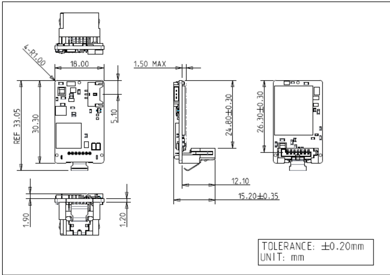
Figure 2: Innodisk SATADOM-SH 3TE7 (BGA) mechanical diagram
