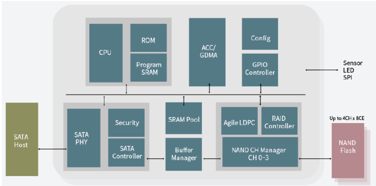
Figure 3: Innodisk SATADOM-SH 3TE7 Block Diagram
