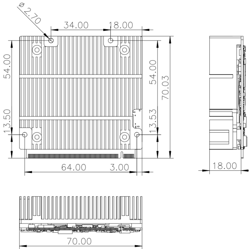
Figure 1-3: iQ7-ASL Dimensions with Heatsink (mm)
