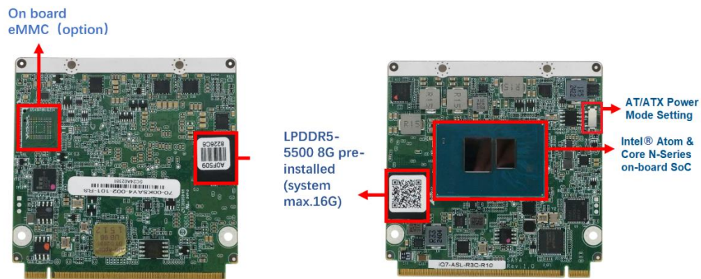
Figure 1-2: On-board Components and Connectors
