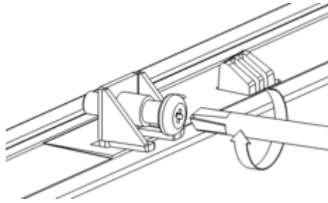
Figure 2.6 Panel Mounting – Clamp Fixing
