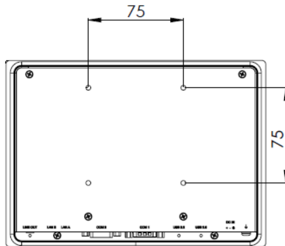
Figure 2.7 VESA Mounting
