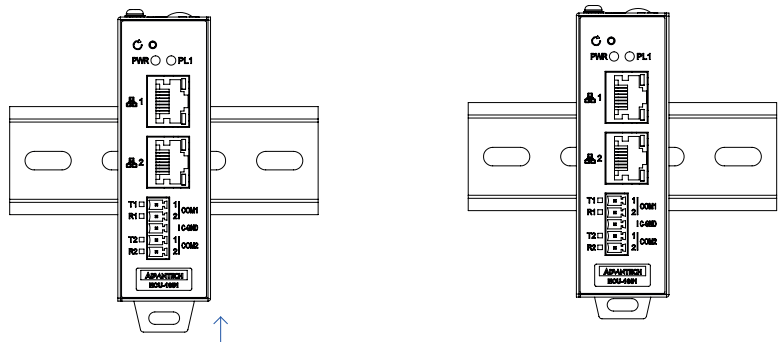
Figure 7. DIN-Rail installation
