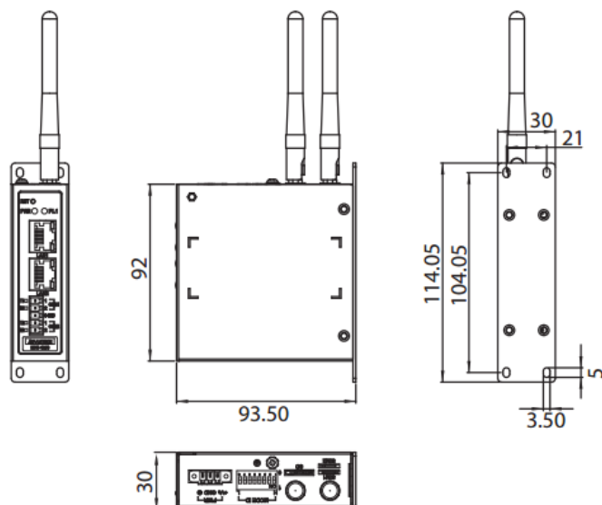
Figure 2. Dimension
