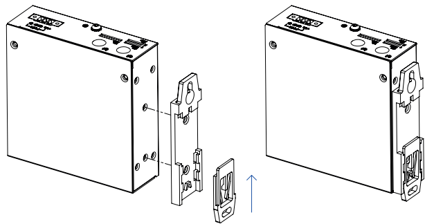
Figure 6. DIN-Rail Kit
