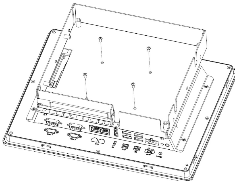
Figure 2.17 PCI/PCle Add-on Box Installation
