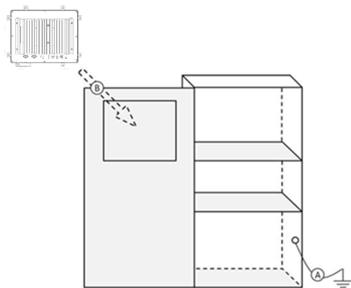
Figure 2.5 Cabinet Installation
