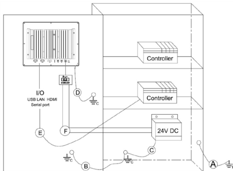
Figure 2.6 System Wiring
