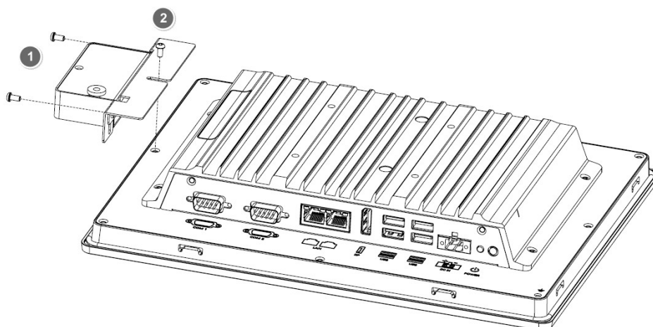
Figure 2.14 RFID Reader Installation
