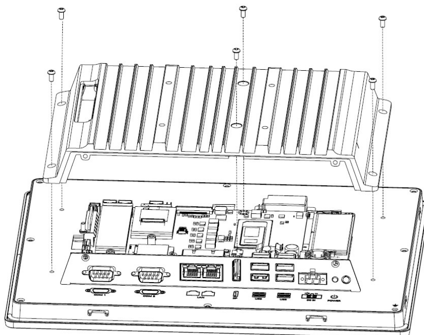
Figure 2.6 Re-installing Rear Cover
