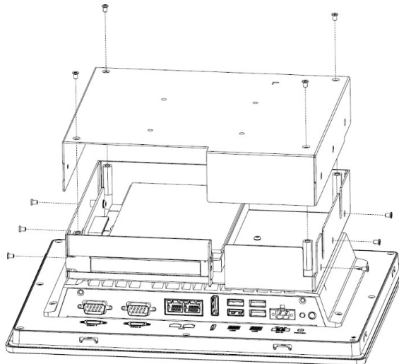
Figure 2.20 Add-on Box Cover Installation
