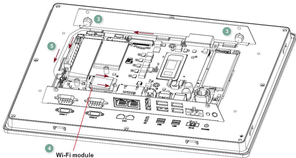
Figure 2.12 Wi-Fi Kit Installation
