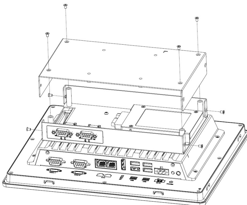
Figure 2.9 Add-on Box Cover Installation
