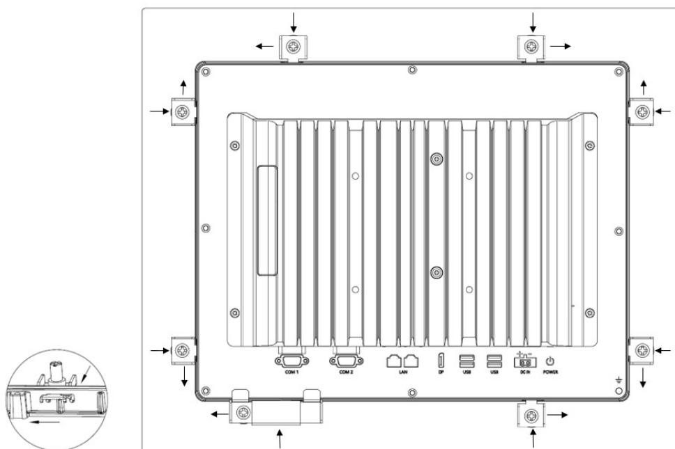
Figure 2.22 Panel Mounting (1)
