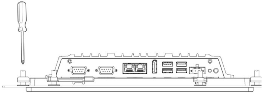
Figure 2.23 Panel Mounting (2)
