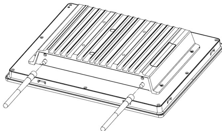
Figure 2.13 External Antenna Installation
