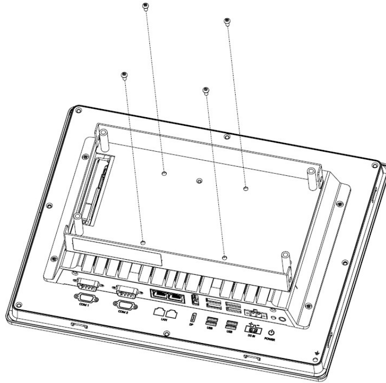
Figure 2.7 SSD/iDoor Add-on Box Installation
