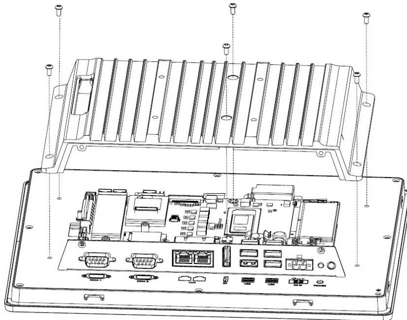
Figure 2.16 Installing the Rear Cover
