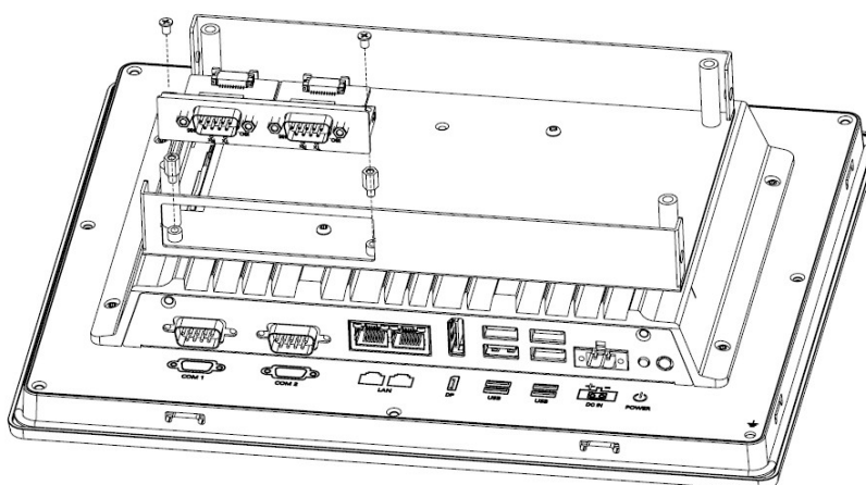
Figure 2.10 iDoor Module Installation
