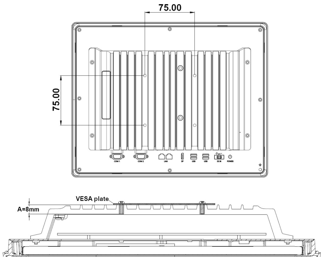
Figure 2.4 VESA Mounting
