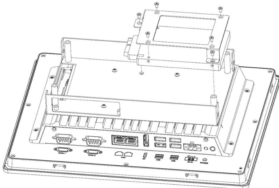
Figure 2.8 SSD Installation
