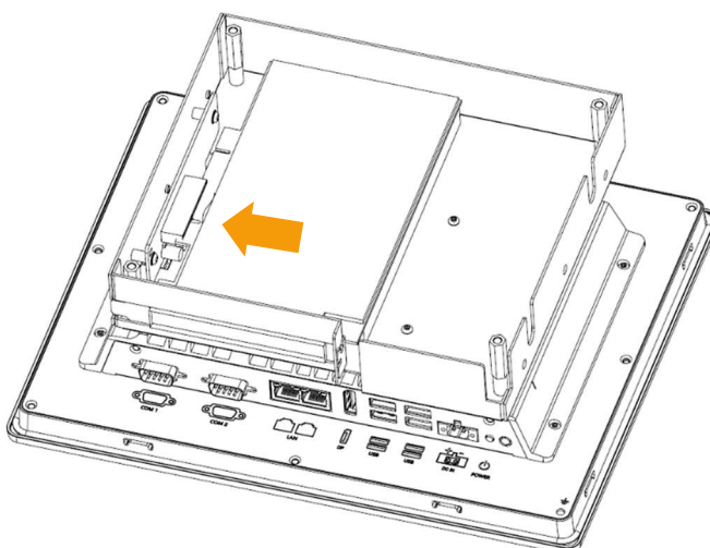
Figure 2.19 Installing PCIe Expansion Card
