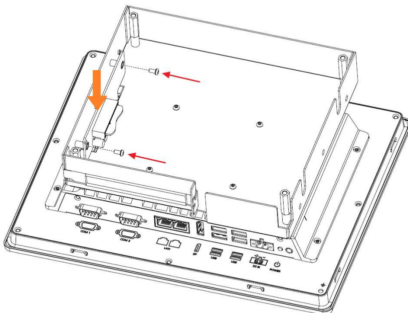
Figure 2.18 Installing a Riser Card
