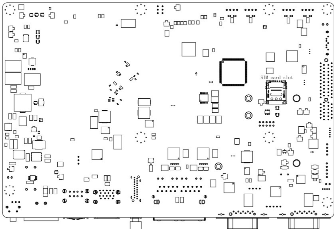
Figure A1.2 Board Layout - Bottom View
