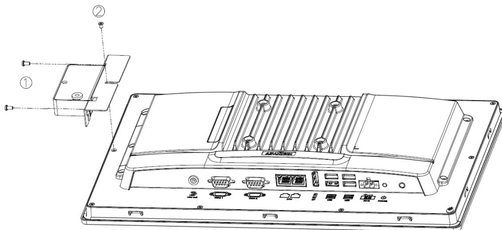
Figure 2.14 RFID Reader Installation
