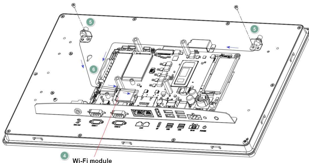
Figure 2.12 Wi-Fi Kit Installation
