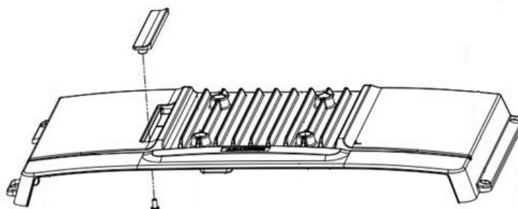
Figure 2.15 PCIe Slot Cover Removal
