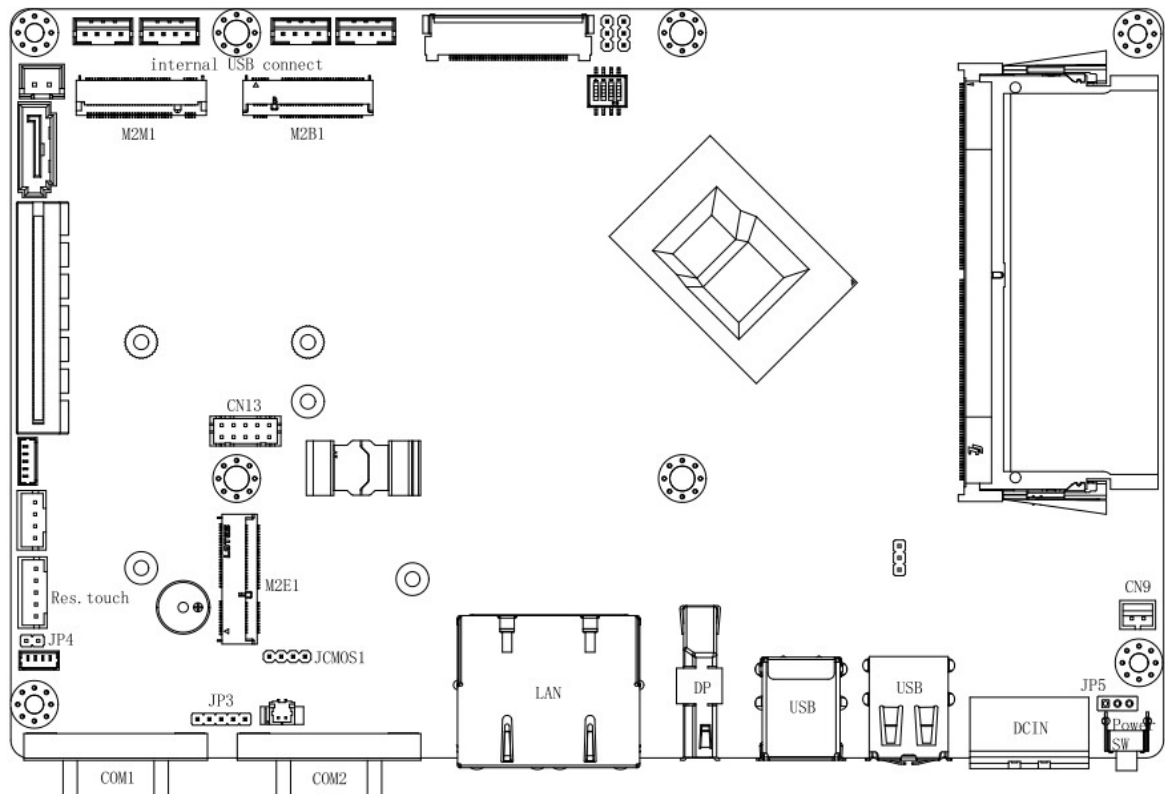
Figure A1.1 Board Layout - Top View
