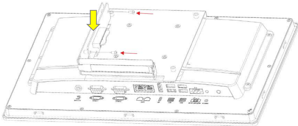
Figure 2.18 Installing a Riser Card
