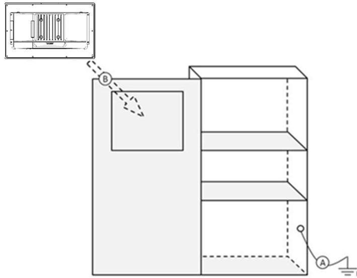
Figure 2.25 Cabinet Installation
