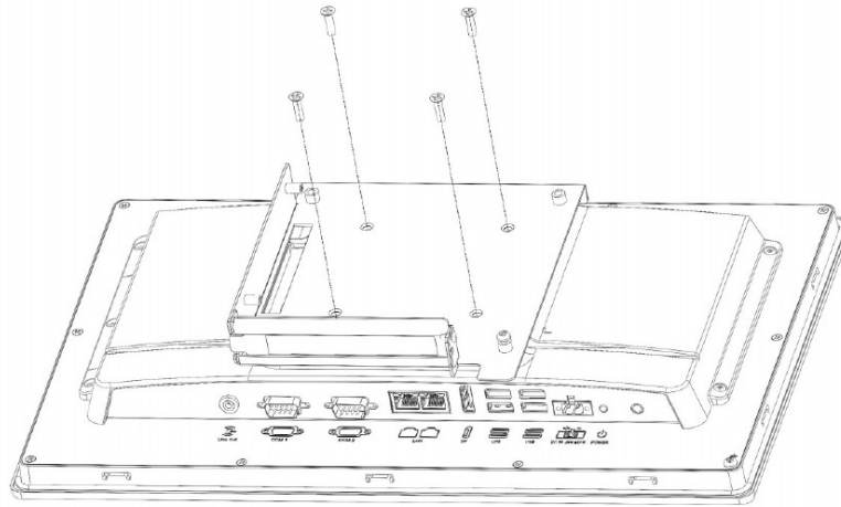
Figure 2.17 Expansion Bracket Installation
