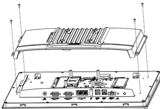
Figure 2.16 Installing the Rear Cover
