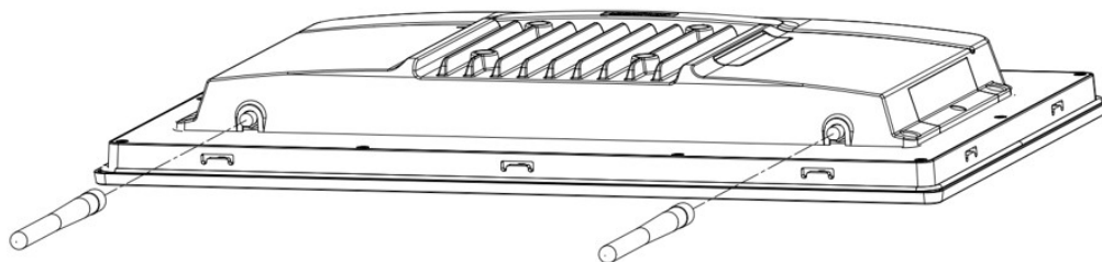
Figure 2.13 External Antenna Installation
