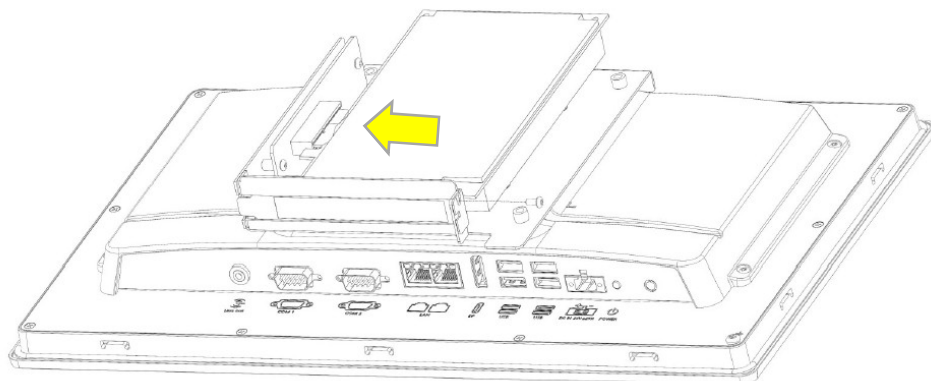
Figure 2.19 Installing PCIe Expansion Card
