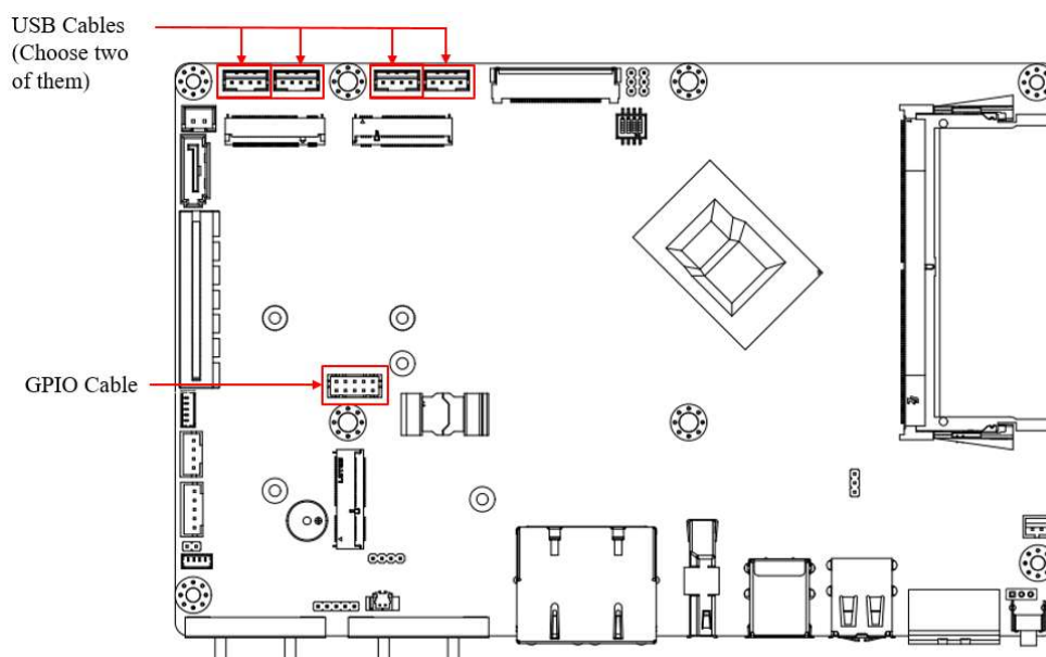
Figure 2.9 GPIO and USB Connectors
