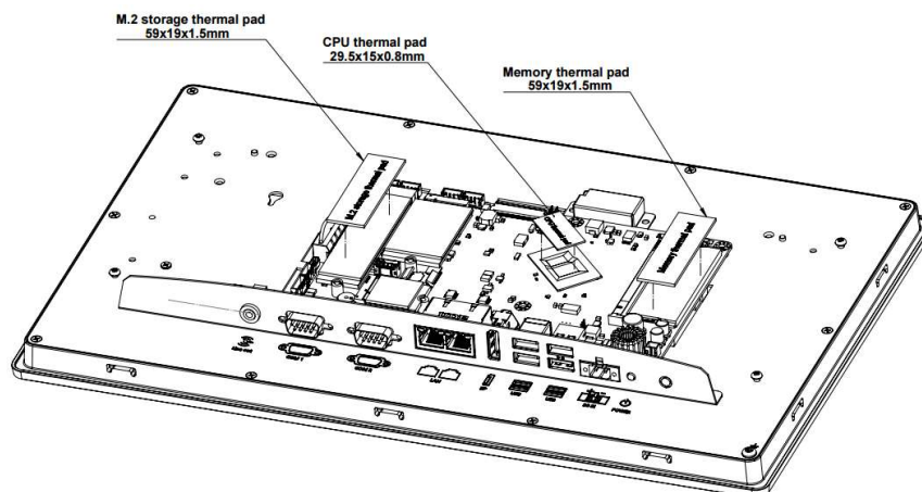
Figure 2.4 Thermal Pad Location
