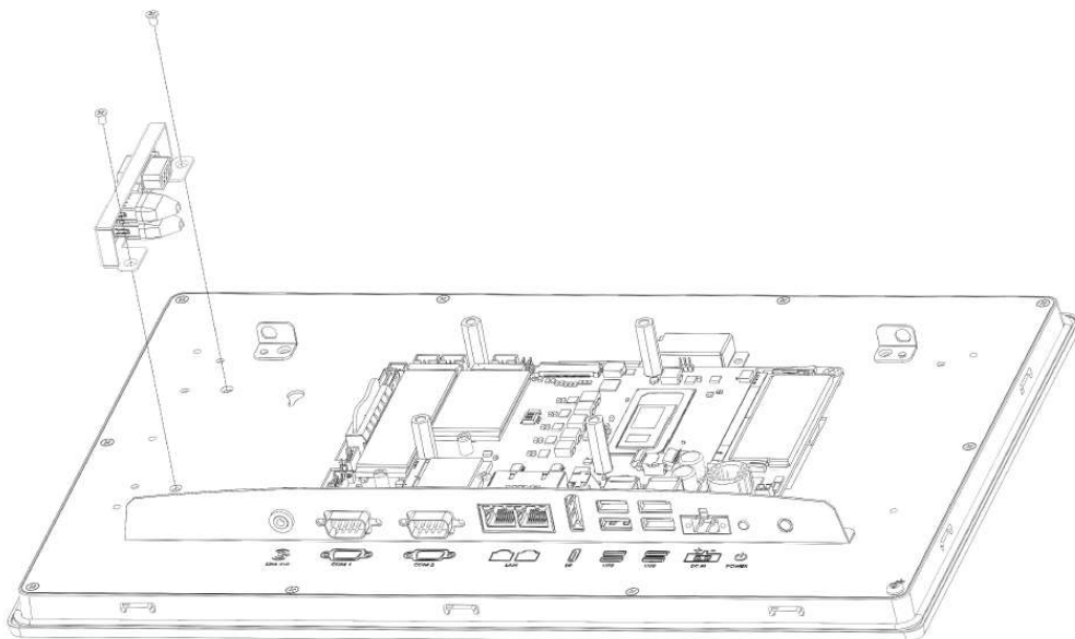
Figure 2.8 GPIO+USB Module Installation
