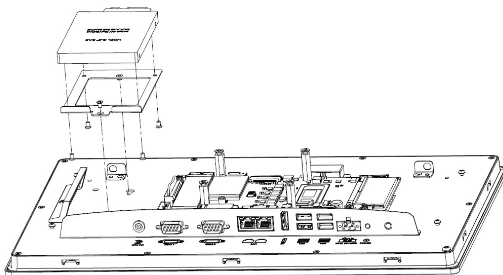
Figure 2.5 SSD Installation
