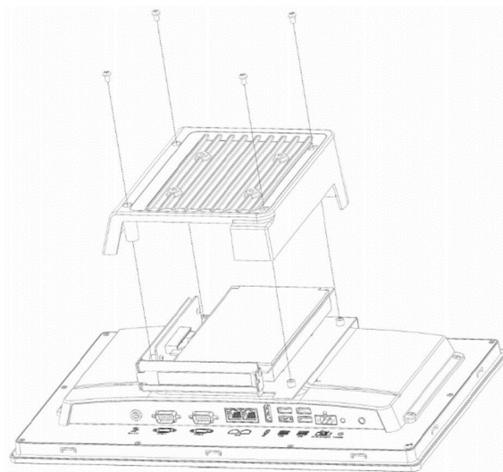
Figure 2.20 Expansion Cover Installation
