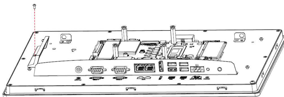
Figure 2.6 iDoor Blank Cover Removal
