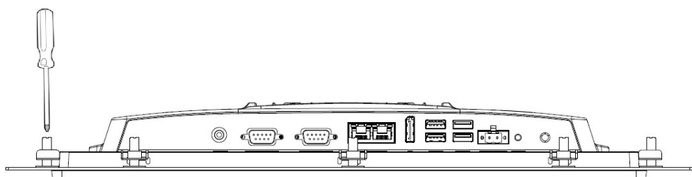
Figure 2.23 Panel Mounting (2)
