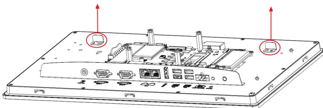
Figure 2.10 Removing Blank Brackets
