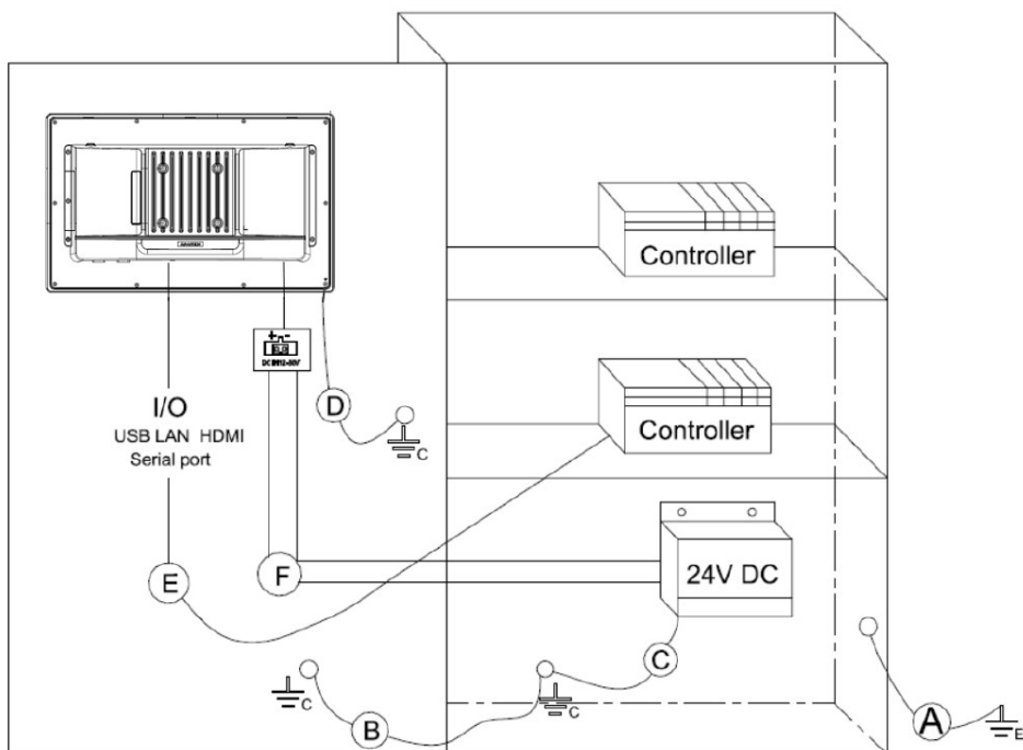
Figure 2.26 System Wiring
