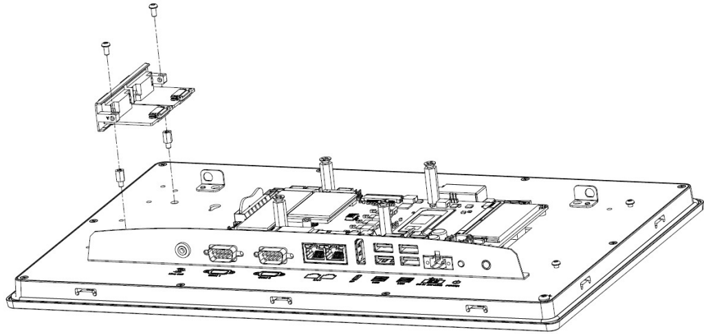
Figure 2.7 iDoor Module Installation
