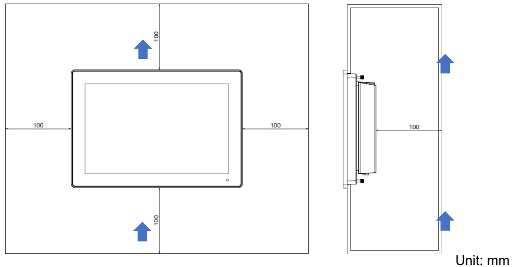
Figure 2.21 Panel Mounting – Positioning
