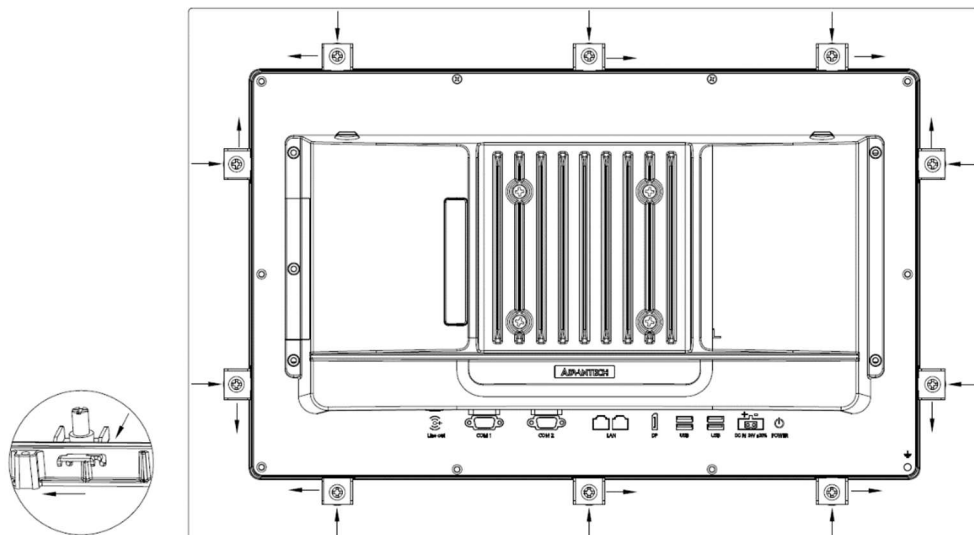
Figure 2.22 Panel Mounting (1)
