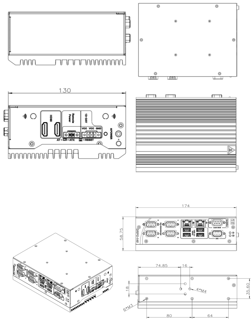
Figure 1-4: Physical Dimensions
