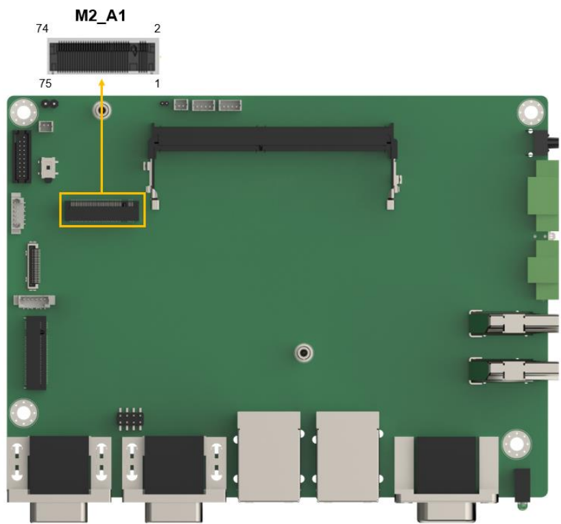
Figure 4-17: M.2 A-key Slot Location
