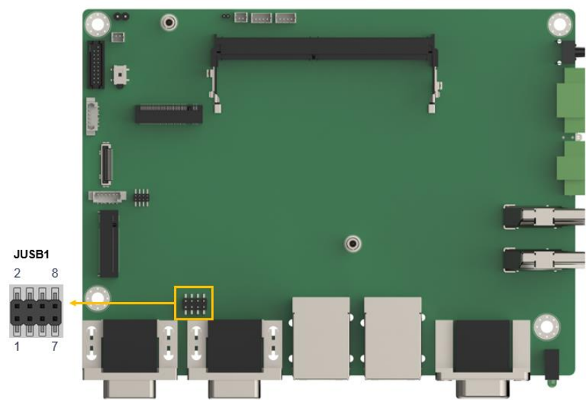
Figure 4-15: Internal USB 2.0 Connectors Locations
