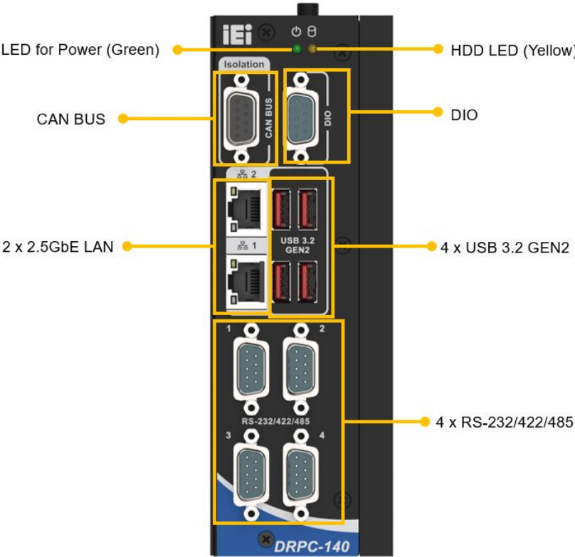
Figure 1-2: Front Panel
