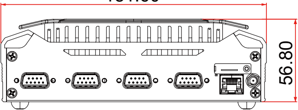
Rear View
