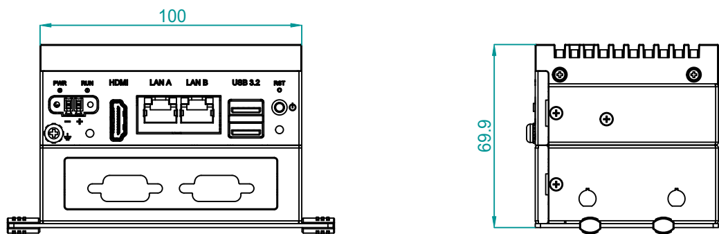
Figure 1.3 UNO-2271G V2 Dimensions (with Stack Extension Kit for iDoor)
