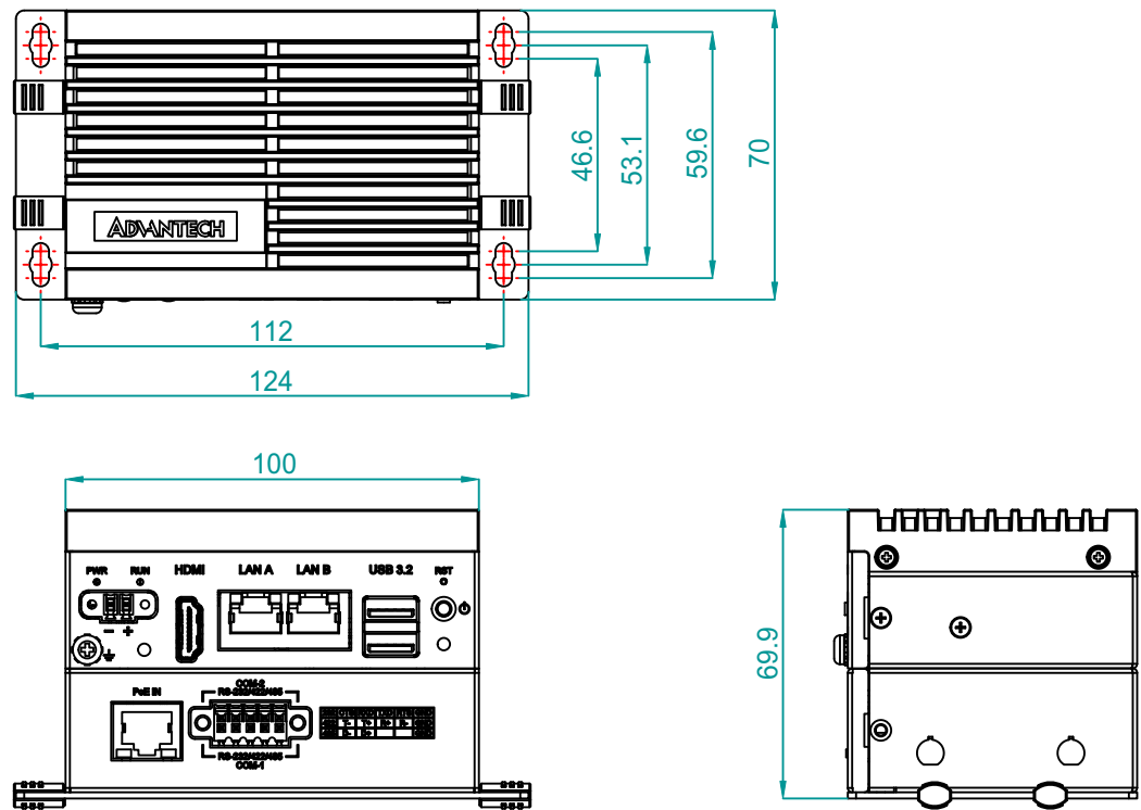
Figure 1.2 UNO-2271G V2 Dimensions (with Optional Extension Kit)
