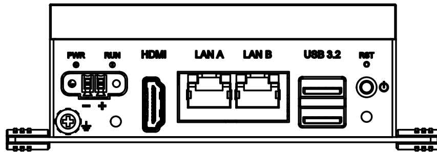
Figure 3.1 Chassis Grounding Connection Diagram
