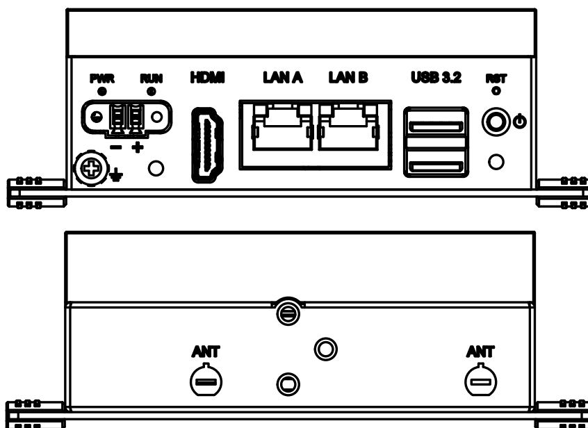
Figure 2.9 LED Indicators, Reset Buttons, and Antenna Hole
