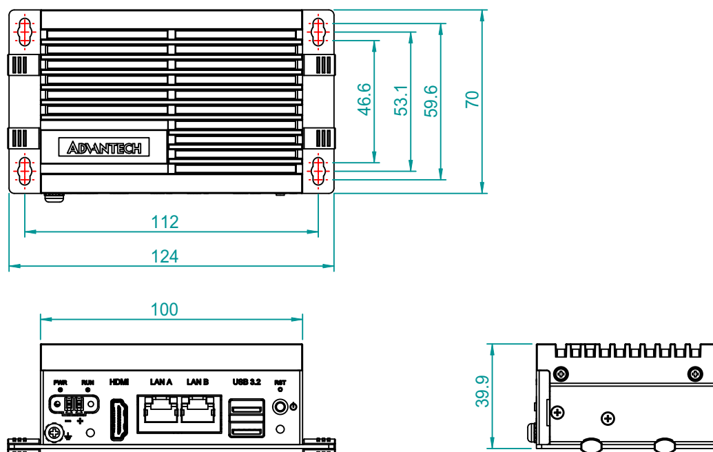
Figure 1.1 UNO-2271G V2 Dimensions
