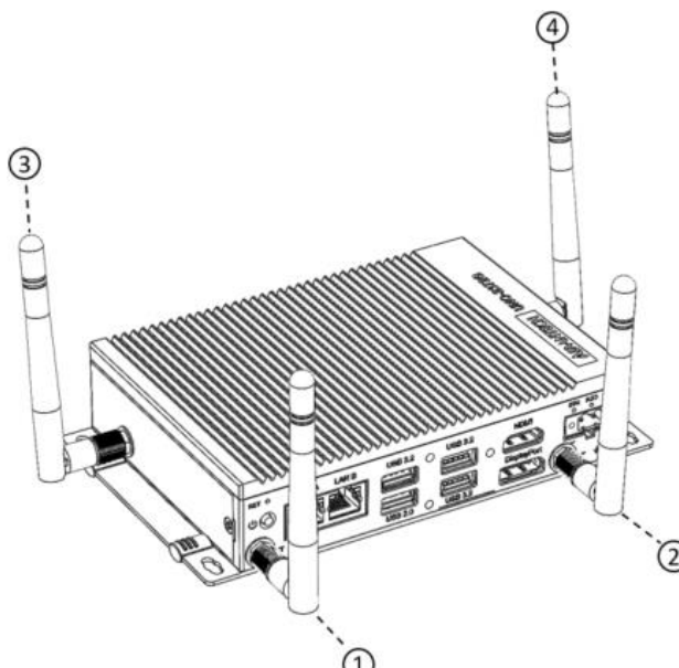
Base unit with 4 antenna
