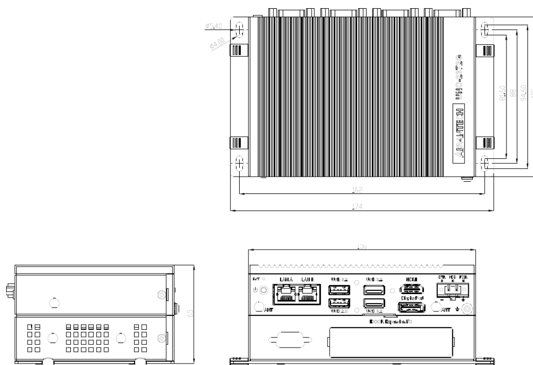
Figure 1.2 UNO-2372G V2 Dimensions (with Optional Extension Kit)
