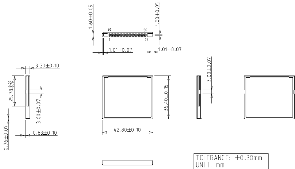
Figure 1: Mechanical Dimension of iCF 1SE3
