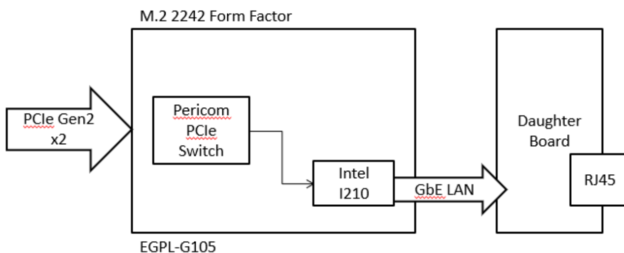
Figure 1: Block Diagram
