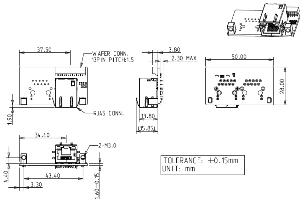
Figure 6: EGPL-G105 M.2 Board Drawing
