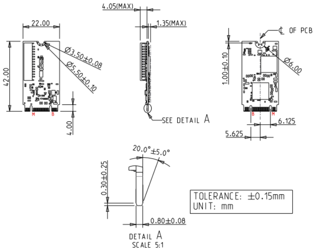
Figure 6: EGPL-G105 M.2 Board Drawing
