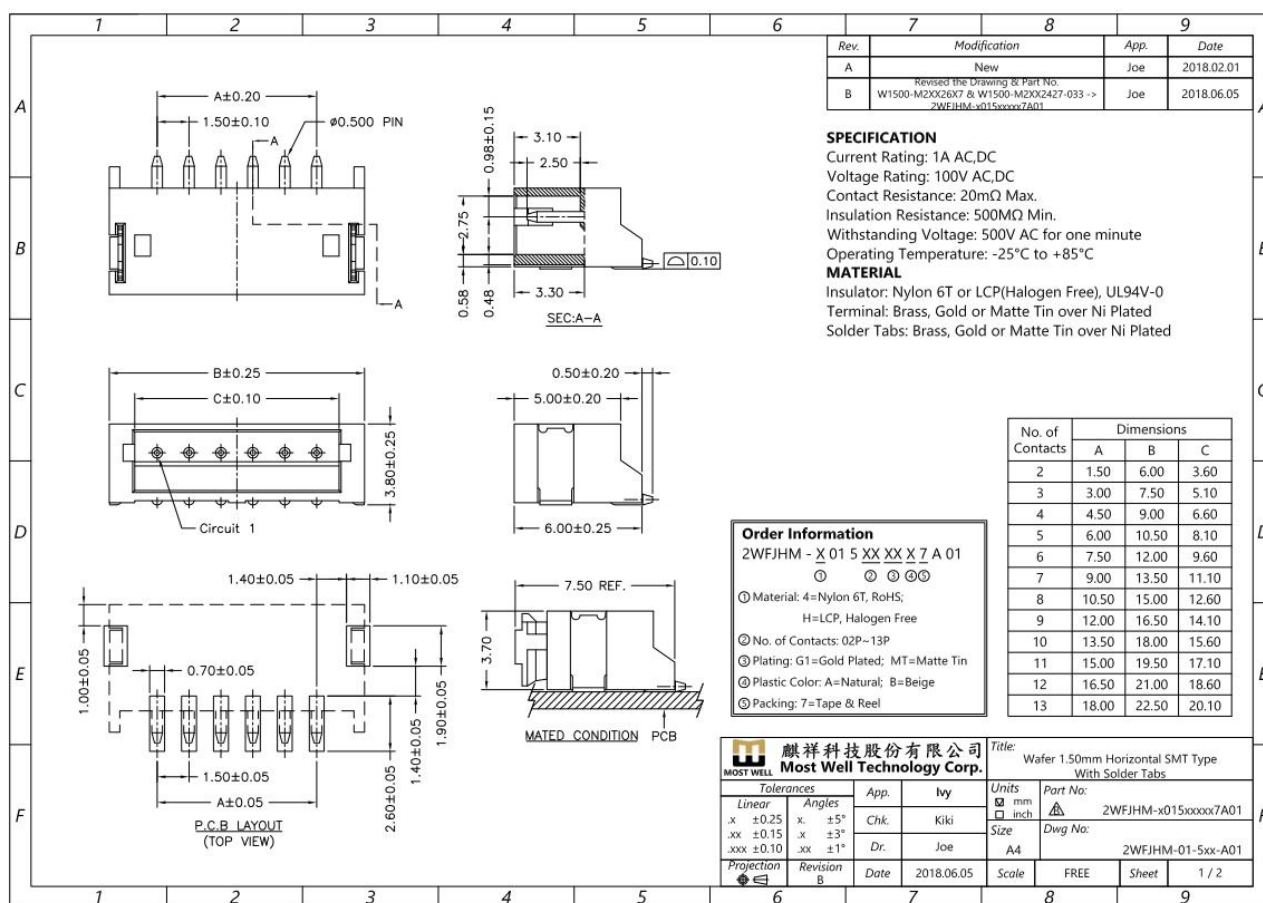
Figure 4: Wire to Board SMD 1*13P Connector Drawing
