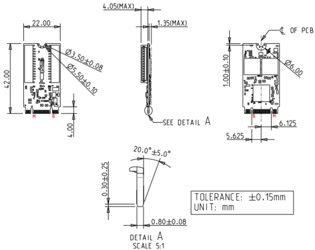
Figure 6: EGPL-G205 M.2 Board Drawing
