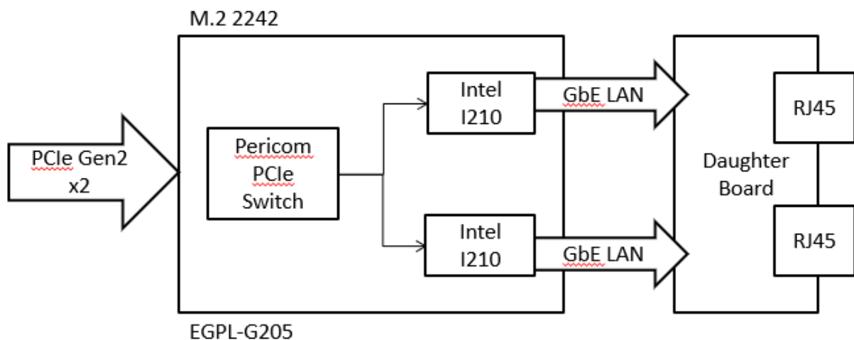
Figure 1: Block Diagram
