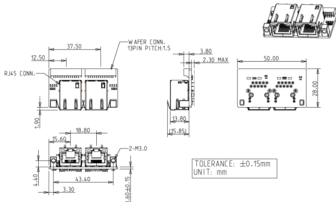
Figure 7: Mounting Hole Daughter Board Drawing (EGPL-G205-C1/W1)
