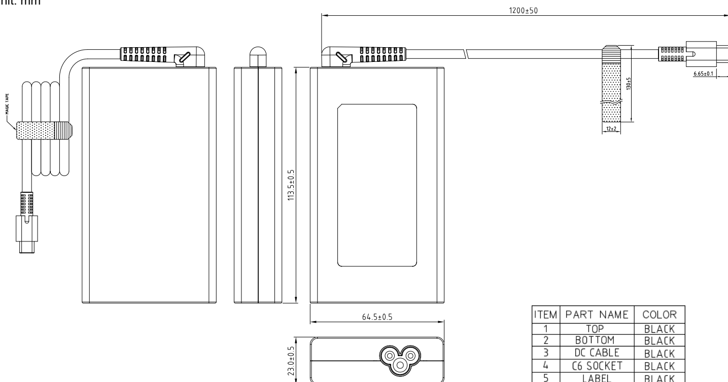
MECHANICAL & AC CONNECTOR SPECIFICATIONS
