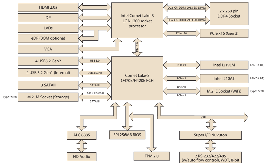
Figure 1.3 AIMB-277 Board Diagram
