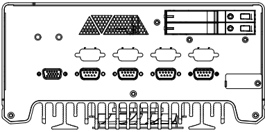
Rear View
