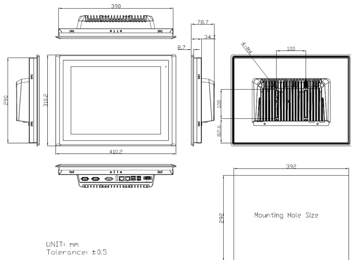
Figure 6 Dimensions of ARCHMI-S-815CP/R
