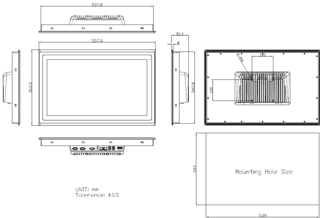
Figure 11 Dimensions of ARCHMI-S-821CP/R
