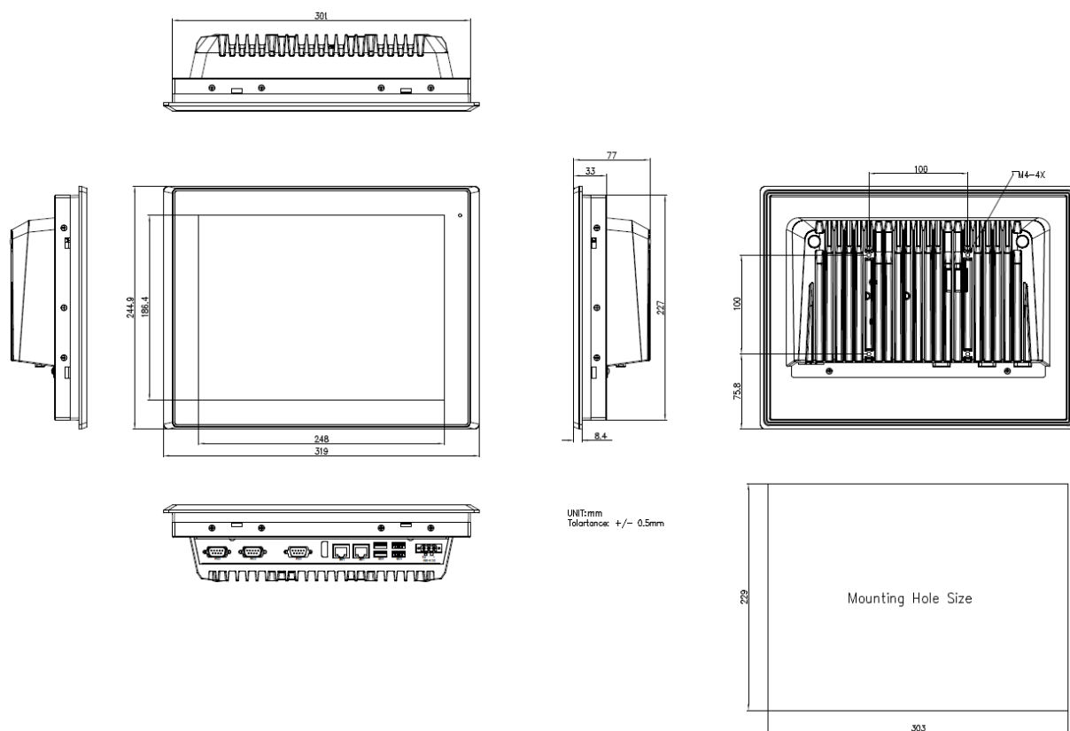
Figure 4 Dimensions of ARCHMI-S-812CP/R
