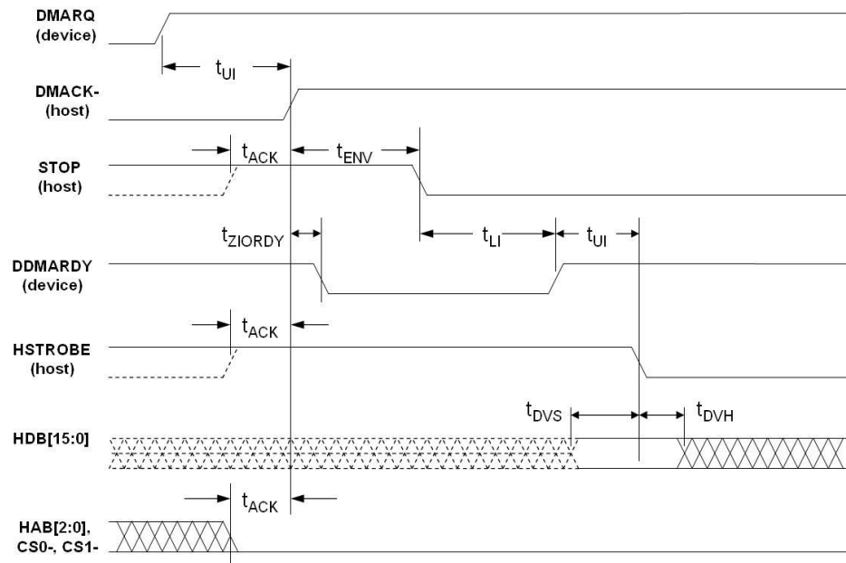
Figure 24: Ultra DMA Mode Data-out Burst Initiation Timing Diagram
