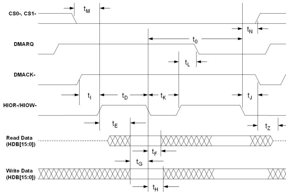
Figure 22: Read/Write Timing Diagram, Multiword DMA Mode
