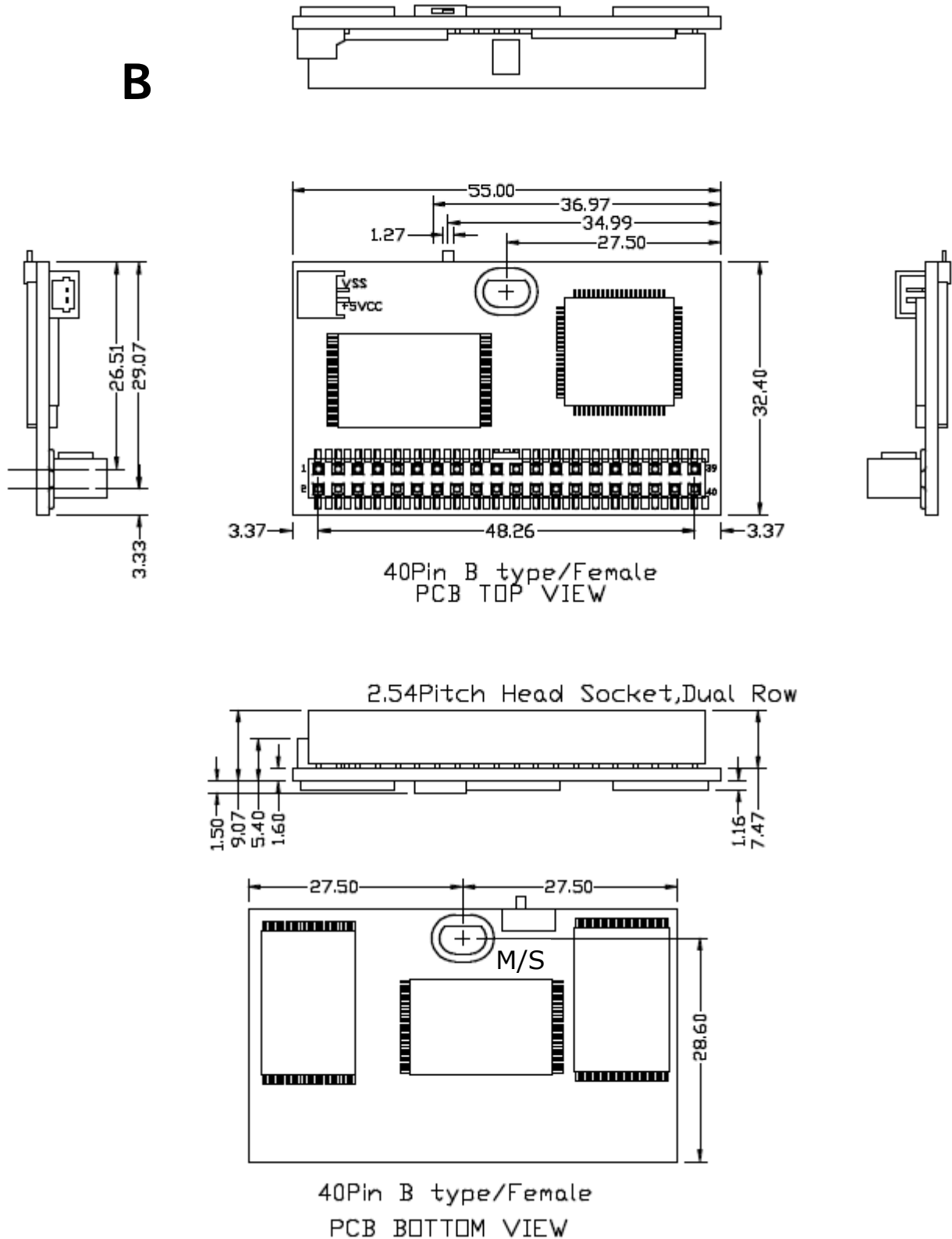
Figure 9: Mechanical Dimension of EDC4000 40-pin(Horizontal Female Type B)
