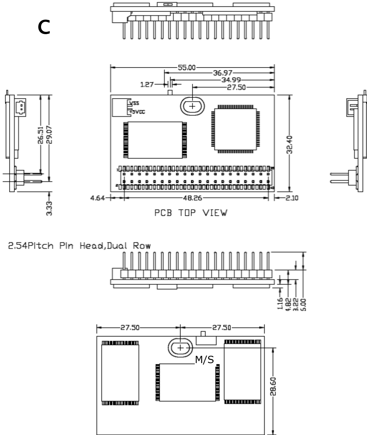
Figure 10: Mechanical Dimension of EDC4000 40-pin(Horizontal Male Type C)
