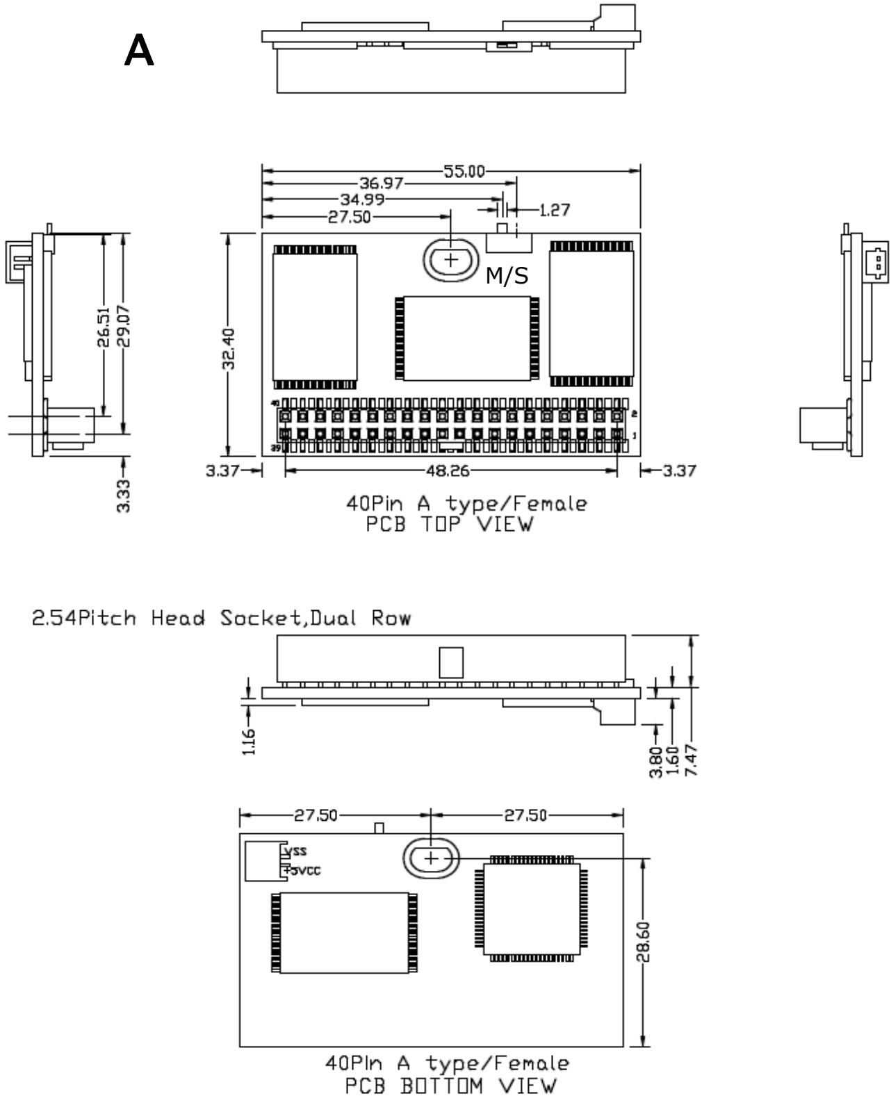
Figure 8: Mechanical Dimension of EDC4000 40-pin (Horizontal Female Type A)
