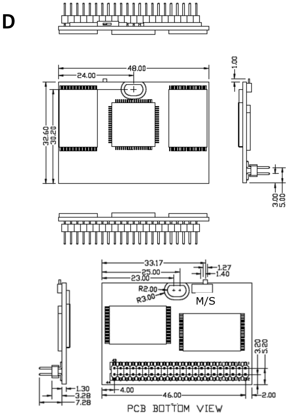
Figure 18: Mechanical Dimension of EDC4000 44-pin (Horizontal Male Type D)
