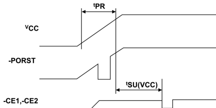
Figure 28 Timing Diagram, Power On Reset
