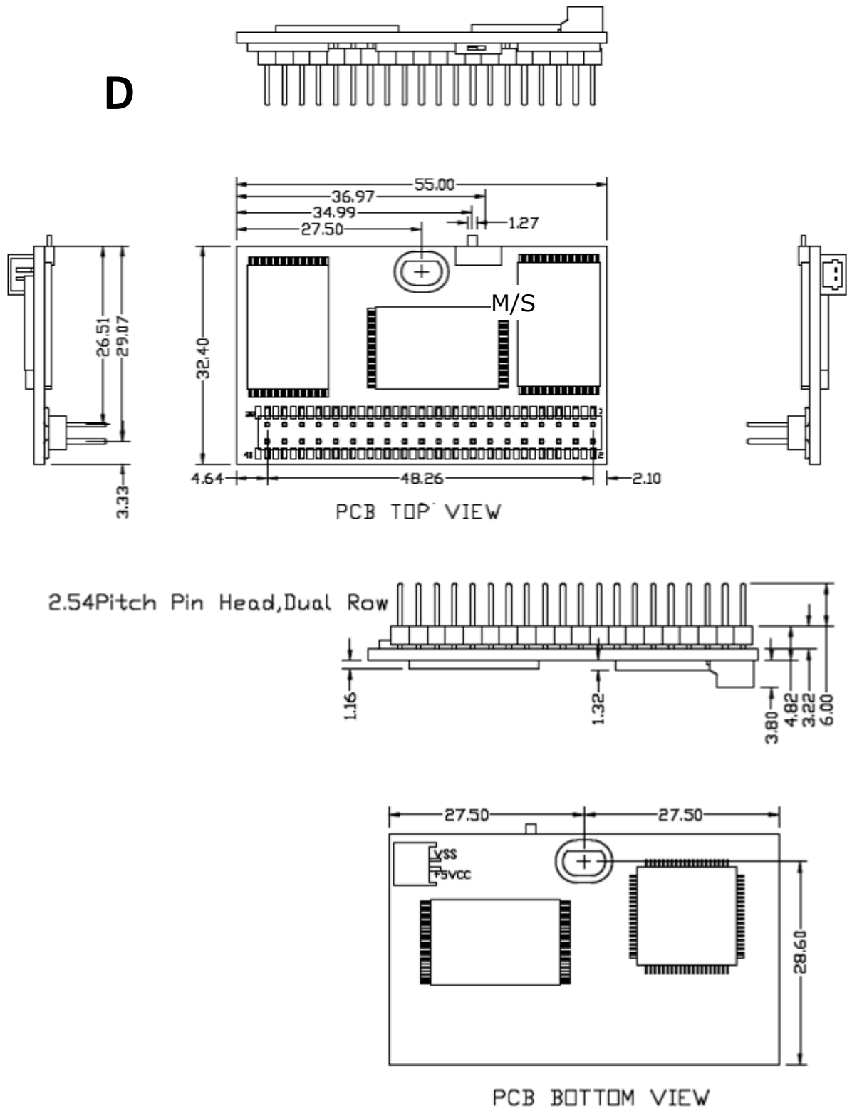
Figure 11: Mechanical Dimension of EDC4000 40-pin(Horizontal Male Type D)
