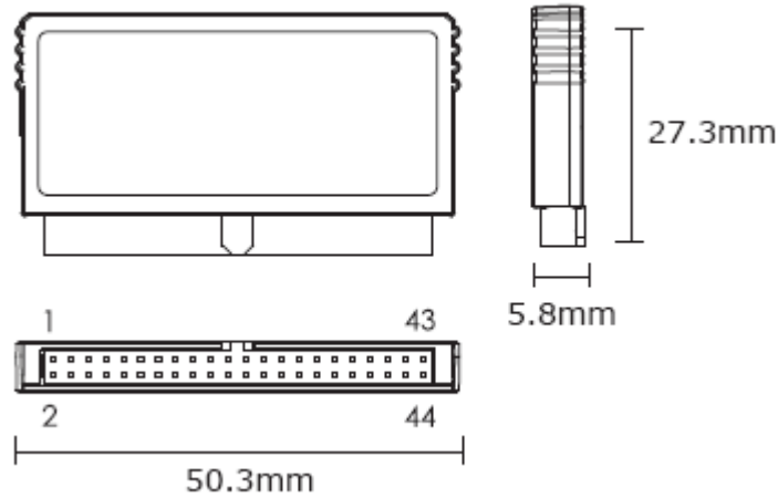
Figure 14: Mechanical Dimension of EDC4000 44-pin (Vertical Version)
