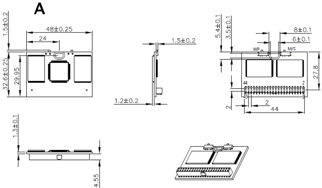
Figure 15: Mechanical Dimension of EDC4000 44-pin (Horizontal Female Type A)
