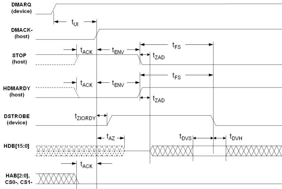
Figure 23: Ultra DMA Mode Data-in Burst Initiation Timing Diagram
