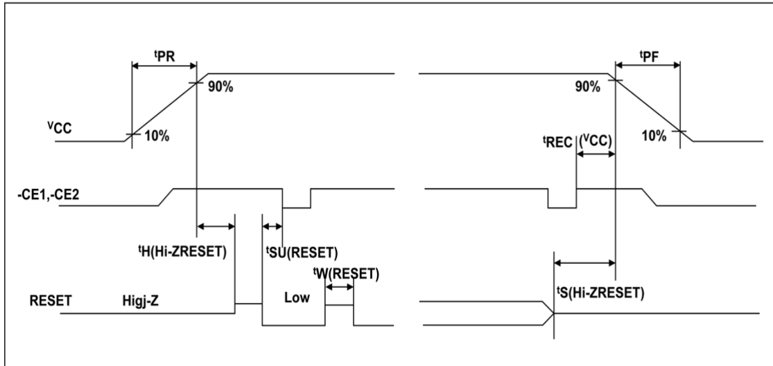
Figure 27 Timing Diagram, Hardware Reset
