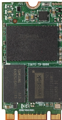
Figure 1: Innodisk M.2 (S42) 3IE2-P (type 2242)
