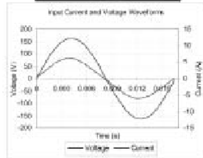
Input AC Current Waveform (THD = 11.99%, 50% Load)
